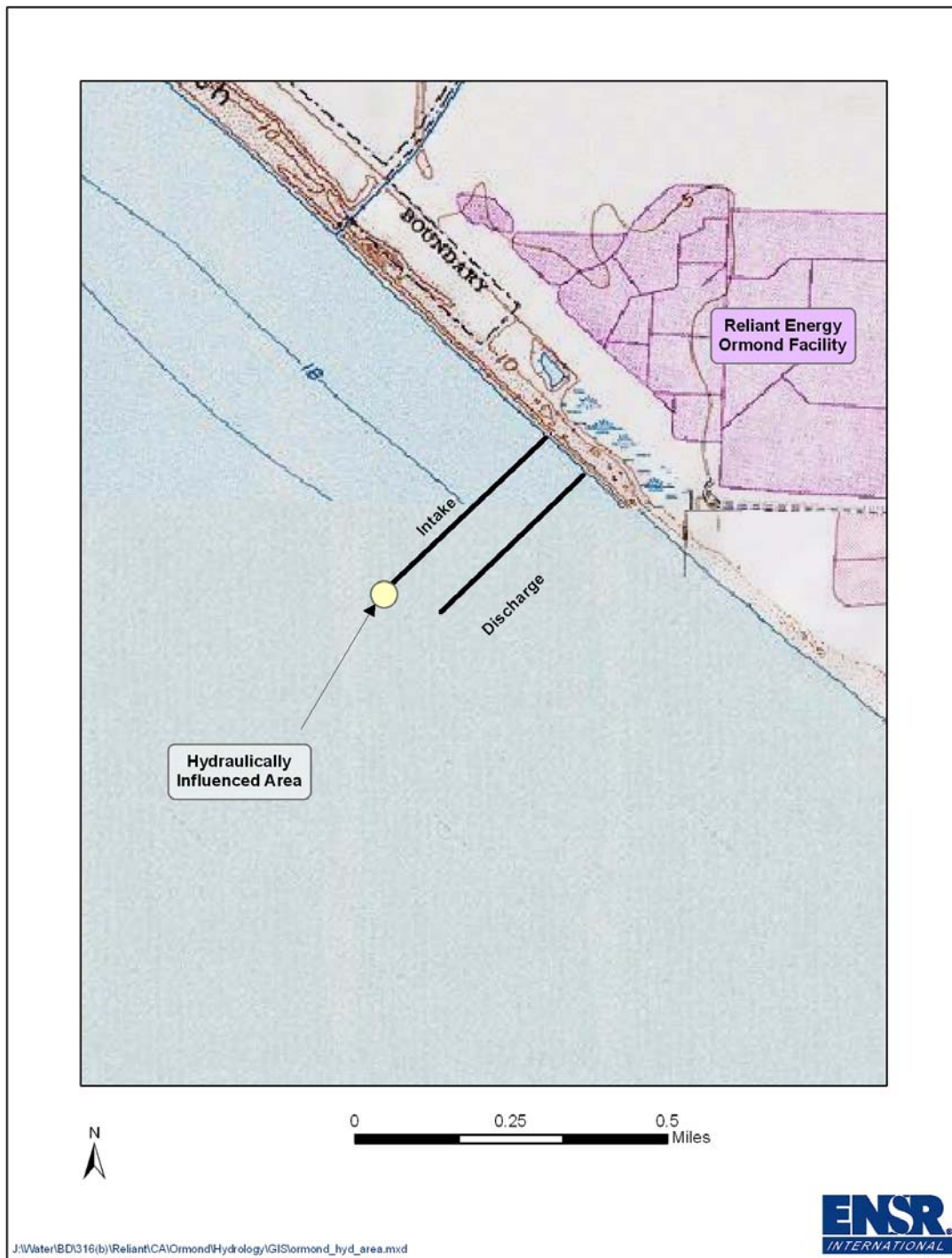
Figure 2-1 Estimated Zone of Hydraulic Influence of the CWIS
