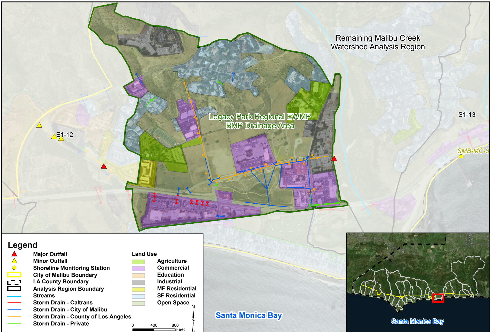
Figure 28. Legacy Park Regional EWMP BMP Drainage Area NSMBCW EWMP RB-AR 5520
