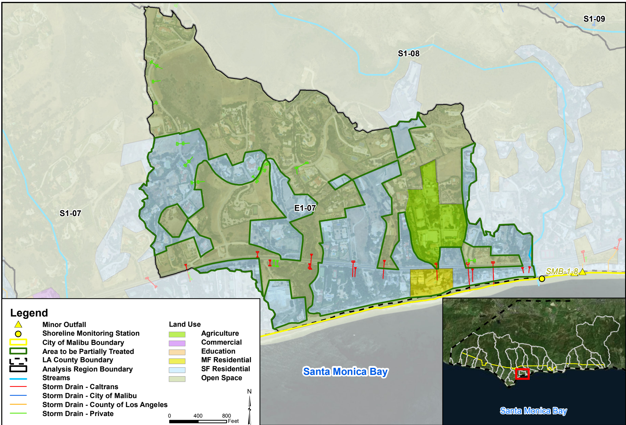
Figure 16. East of Ramirez Creek at Paradise Cove (Analysis Region E1-07) Area to be Treated by Distributed BMPs (35% of Area Outlined in Green) NSMBCW EWP RB-AR 5493
