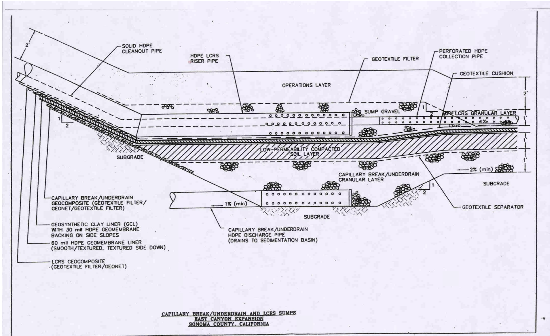
Engineered Alternative Liner System
