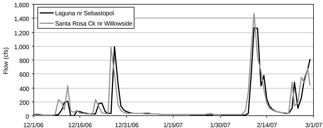
Figure 6. Flows for December 2006 through February 2007 for Laguna near Sebastopol and Santa Rosa Creek at Willowside
