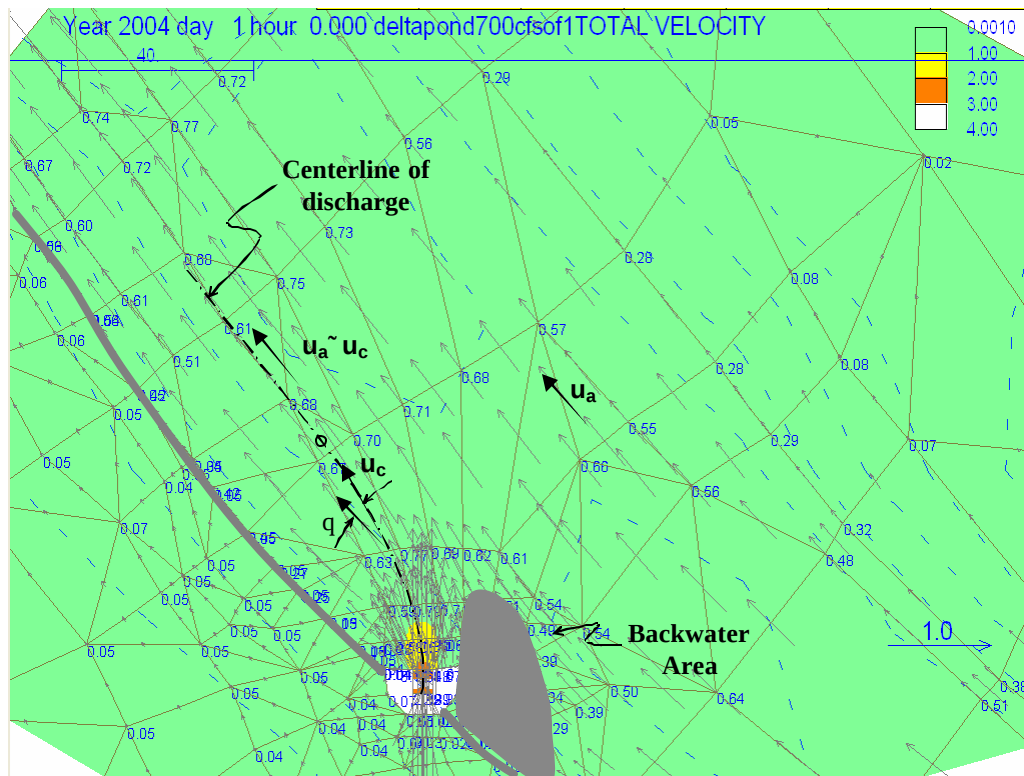
Figure 10. Example RMA-2 velocity vector field showing ambient velocity ( u_a ), centerline jet (discharge) velocity ( u_c ), angle between ambient and centerline velocity ( q ), and location of backwater (gray area) used in determining ZID location
