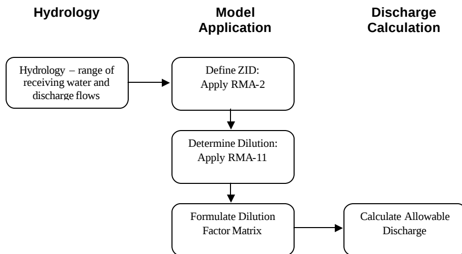
Figure 5. Schematic of process to develop discharge compliance calculator
