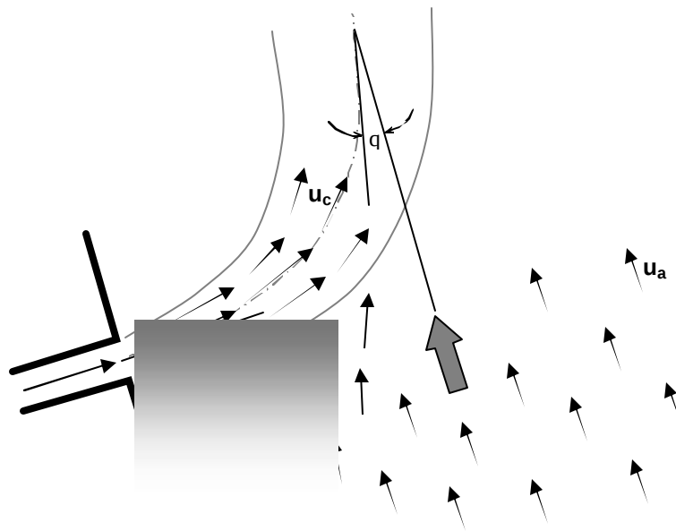
Figure 9. Hypothetical velocity distribution and backwater (in grey) associated with a discharge into a cross current
