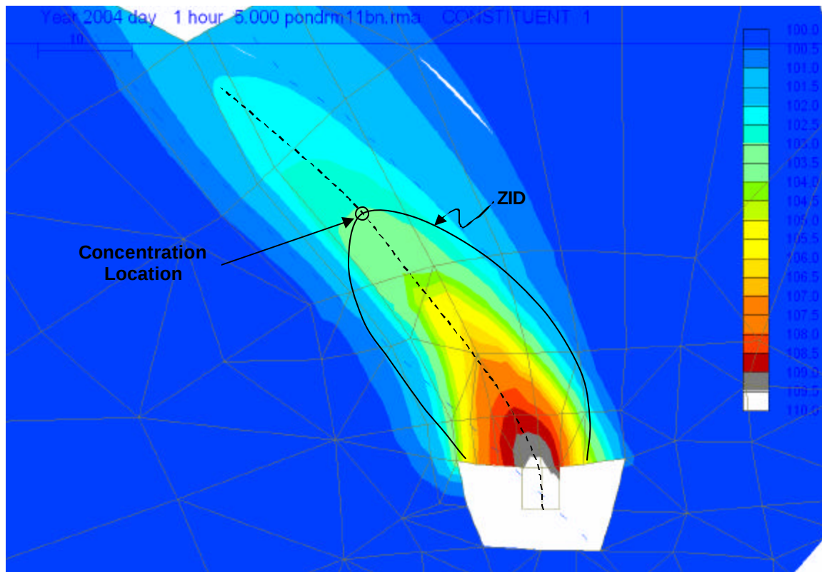
Figure 13. Outfall ZID Boundary Example for flows higher than 400 cfs in Santa Rosa Creek
