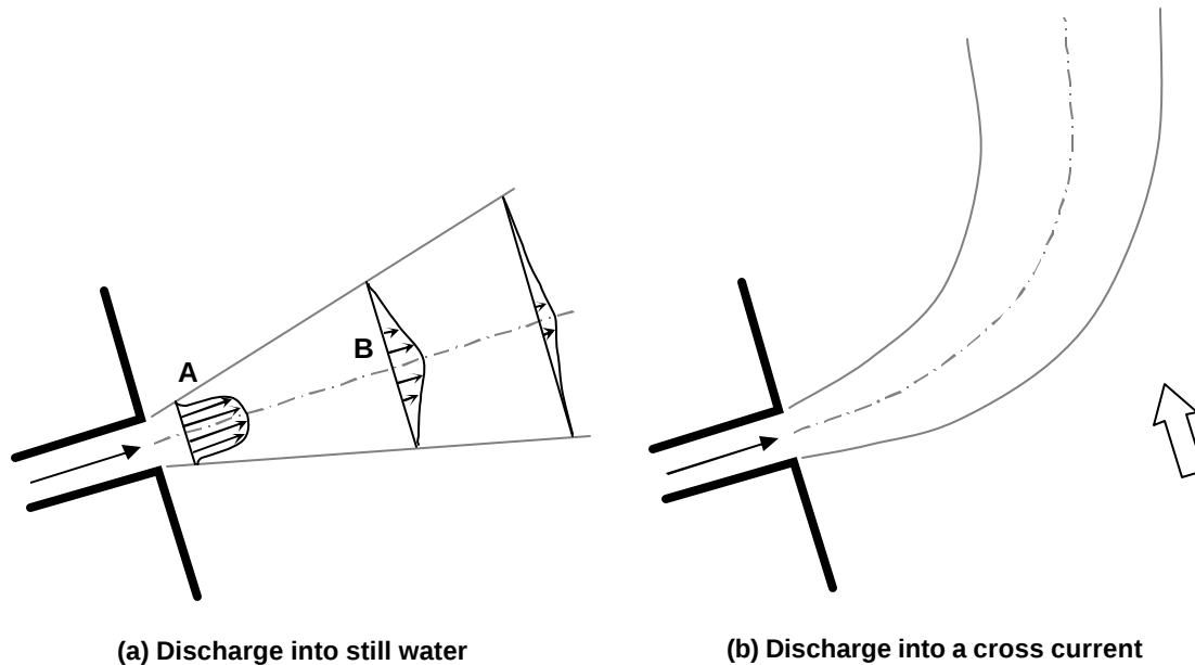
Figure 8. Discharge into (a) still water and (b) a cross current
