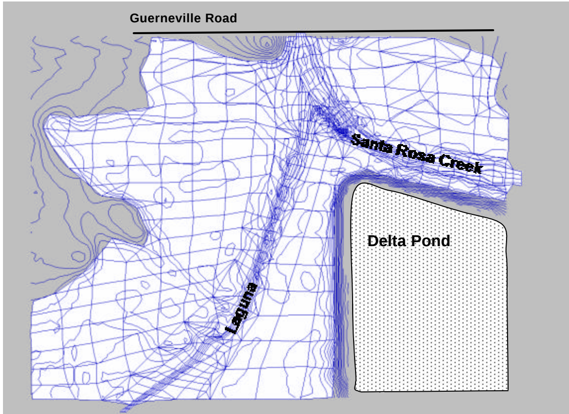
Figure 3. RMA2 Finite Element Mesh
