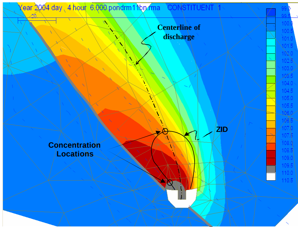
Figure 12. Outfall ZID Boundary Example for Bank Attachment Case
