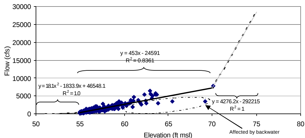
Figure 4. Laguna de Santa Rosa at Guerneville Road stage-discharge relationship
