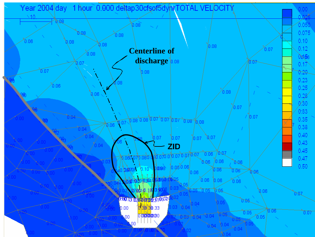
Figure 11. Outfall ZID extend for a 5 cfs discharge into a 30 cfs receiving water flow
