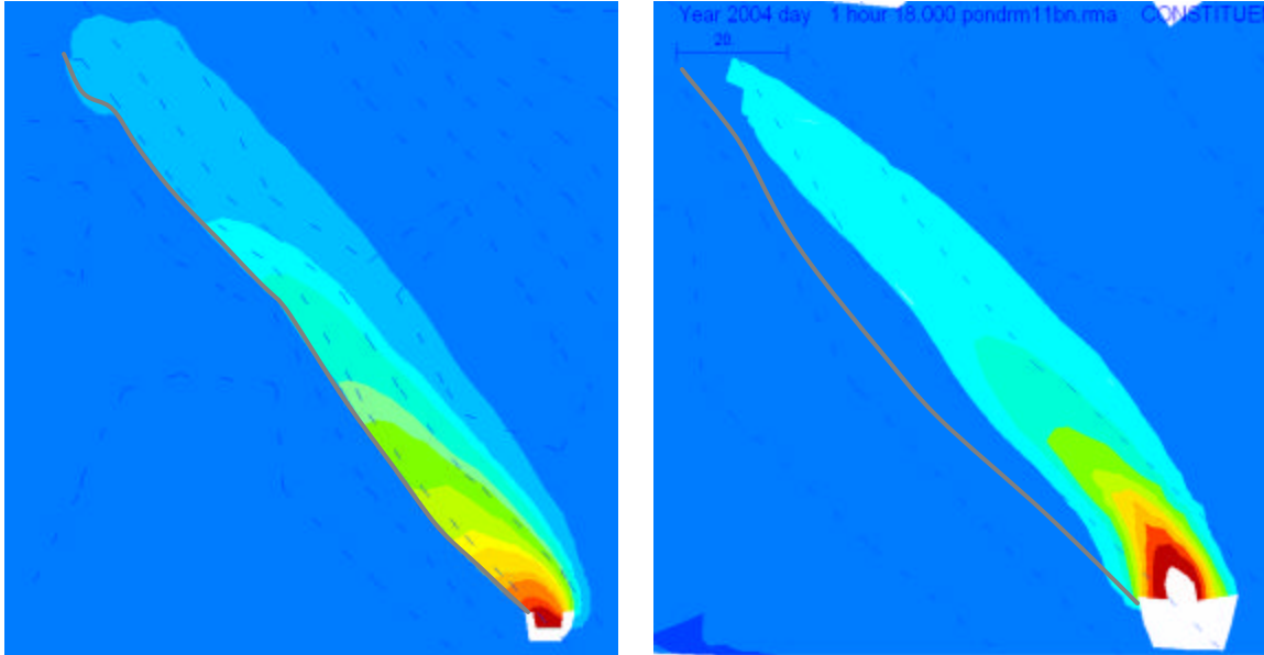
Figure 7. Illustrative concentration gradients for (a) flows lower than 400 cfs in Santa Rosa Creek (bank attachment) and (b) flows greater than 400 cfs in Santa Rosa Creek with contributions from upstream Laguna flows (no bank attachment) [note: approximate shoreline in gray, figures are not on equal scales]
