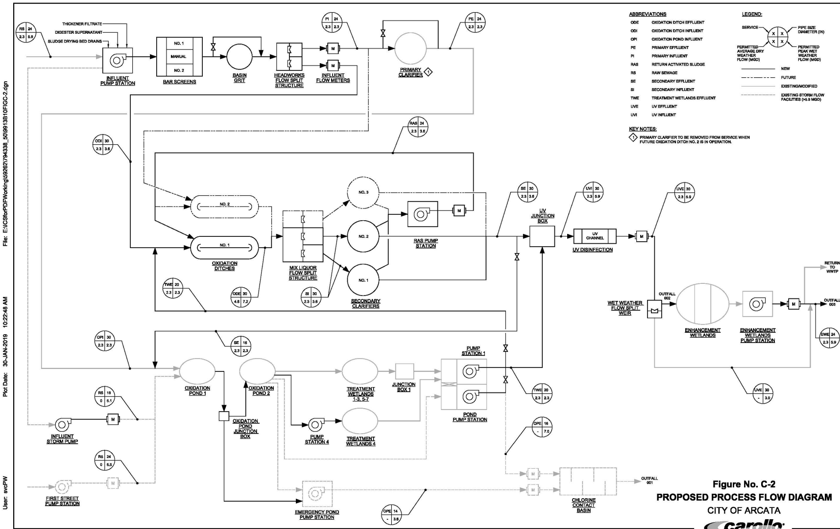
Figure C-2. Proposed Treatment Upgrade Flow Schematic
