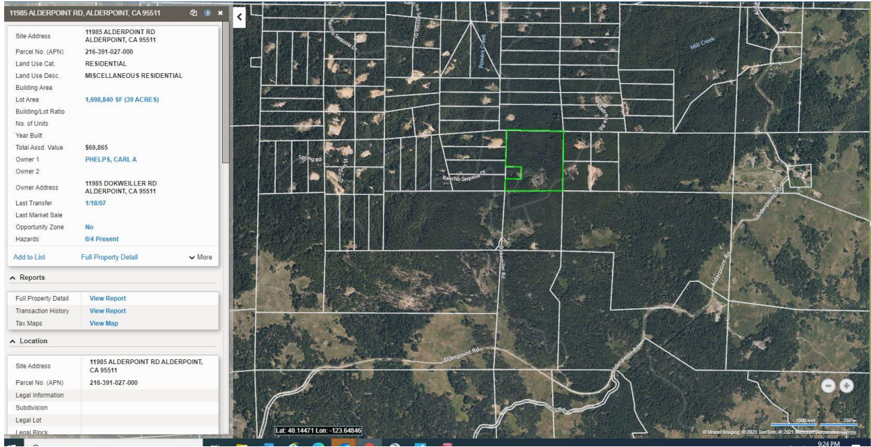
Figure 1. Location map of Property, located south of the Rancho Sequoia subdivision.
