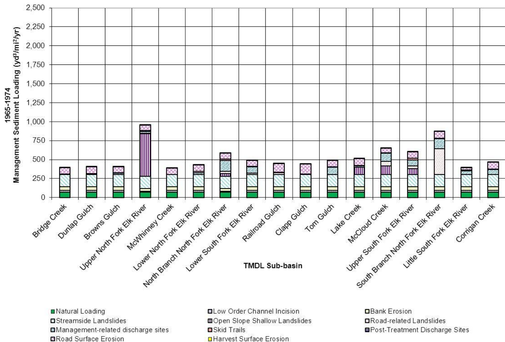
Figure 2. Annual sediment loading by management source category for TMDL subbasins for the 1965-1974 analysis time period.
