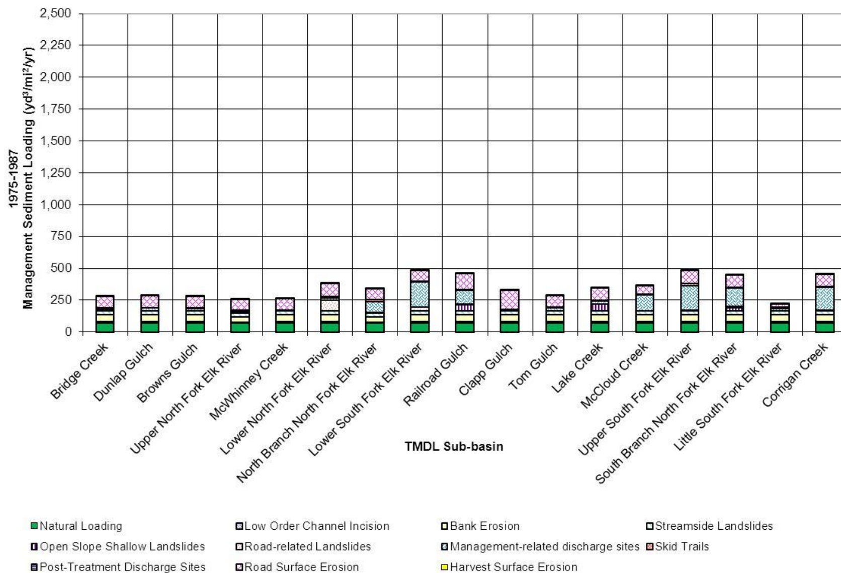
Figure 3. Annual sediment loading by management source category for TMDL subbasins for the 1975-1987 analysis time period.
