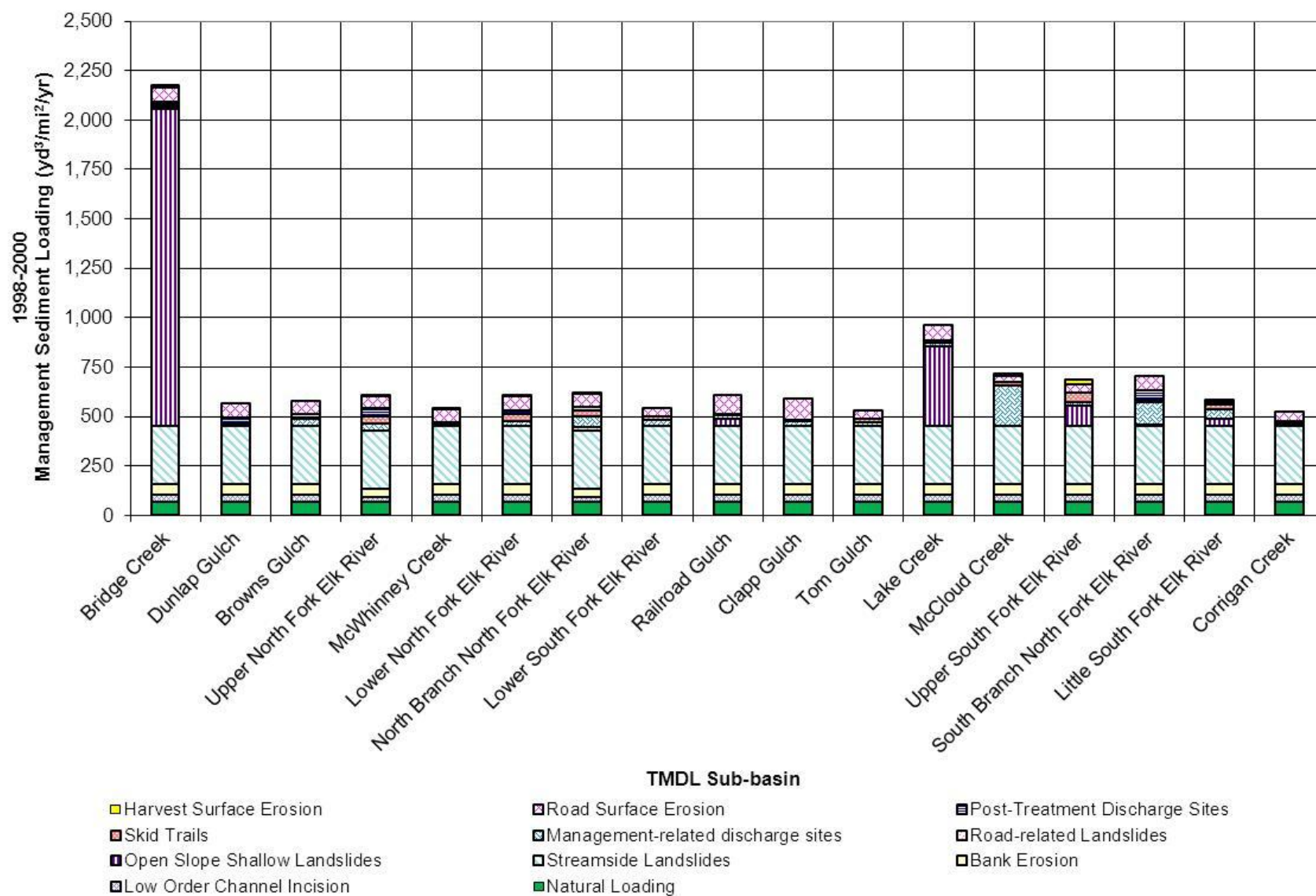
Figure 5. Annual sediment loading by management source category for TMDL subbasins for the 1998-2000 analysis time period.
