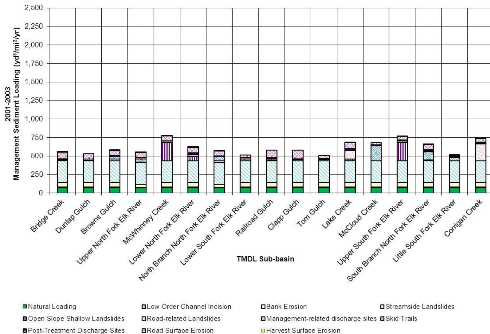
Figure 6. Annual sediment loading by management source category for TMDL subbasins for the 2001-2003 analysis time period.
