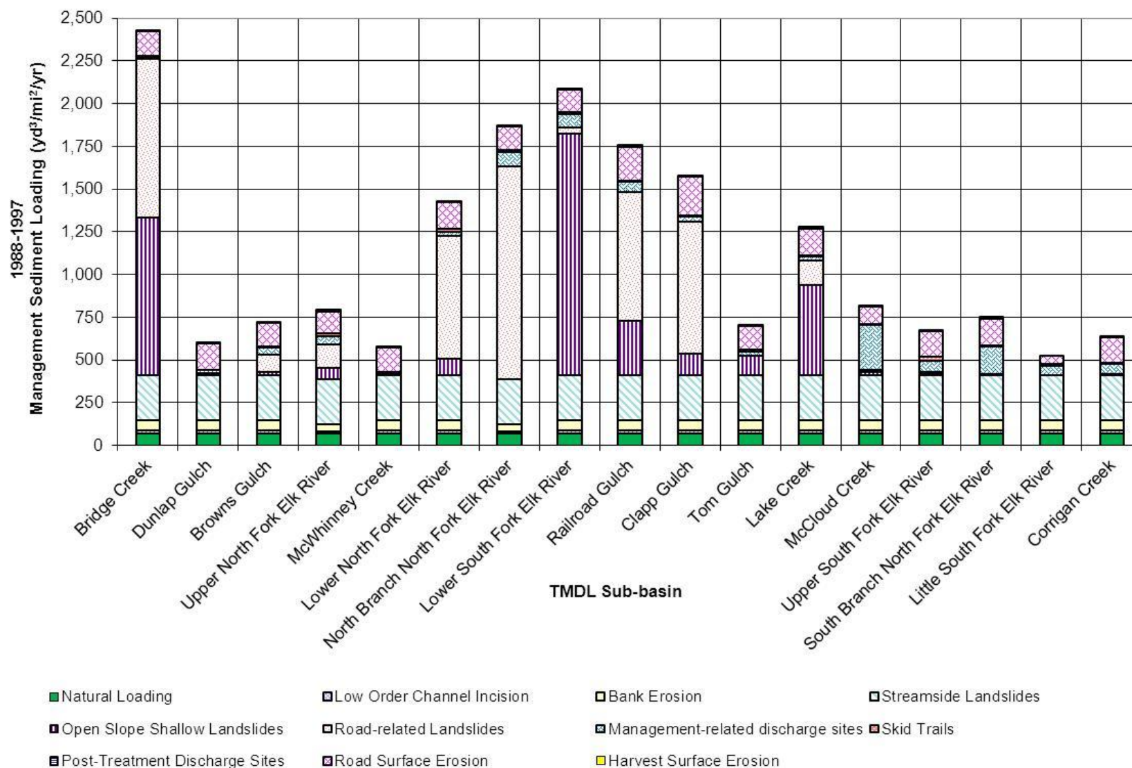
Figure 4. Annual sediment loading by management source category for TMDL subbasins for the 1988-1997 analysis time period.
