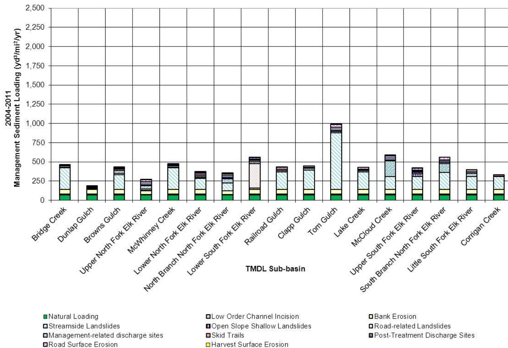
Figure 7. Annual sediment loading by management source category for TMDL subbasins for the 2004-2011 analysis time period.
