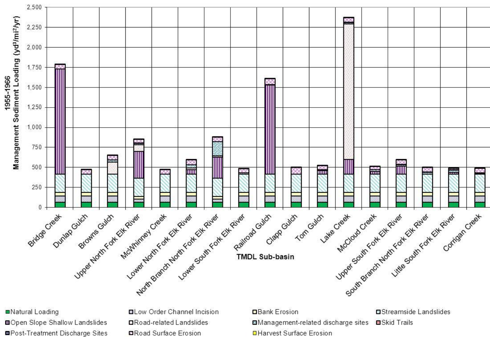
Figure 1. Annual sediment loading by management source category for TMDL subbasins for the 1955-1966 analysis time period.
