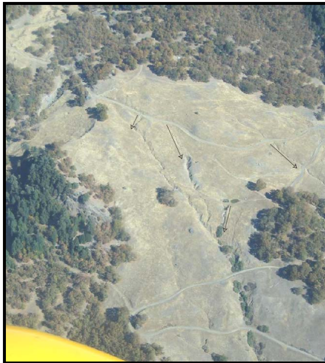
Photograph 3. Earthflow in mélange with private road dissecting the slide looking oblique to the north west. Surface runoff from roads causing large gully erosion below road prism (arrows) and enlarging intermittent channels relative to channels upstream of road.
