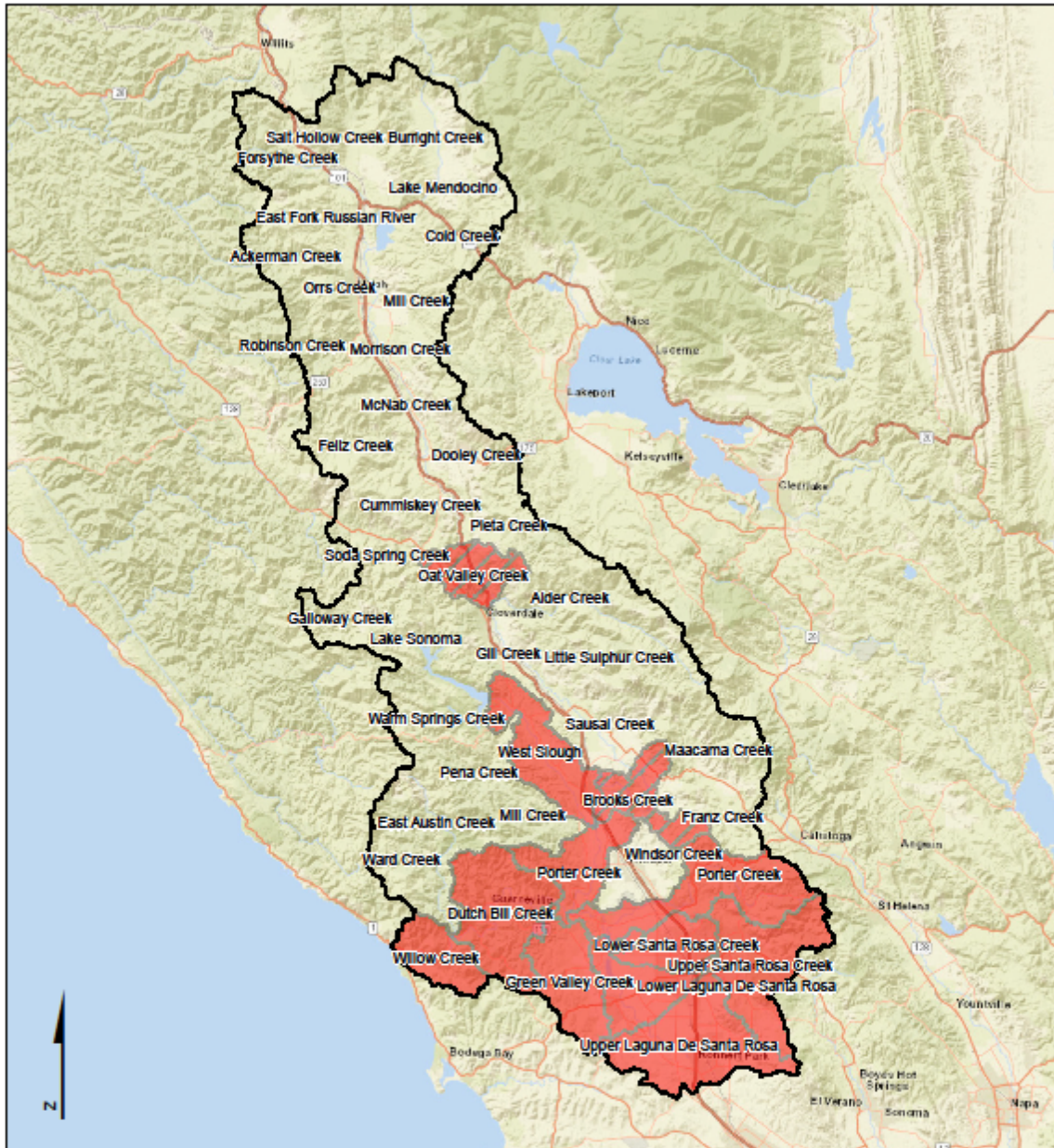
Impairment/Pollution based on Exceedance of Statewide Bacteria Objectives Impairment/Pollution based on Exceedance of U.S. E.P.A. Bacteria Objectives for Enterococci + Public Health Advisories 10 5 0 10 20 Miles 10 5 0 10 20 Kilometers Russian River Watershed HUC-12 Subwatersheds with Direct Evidence of Impairment/Pollution
