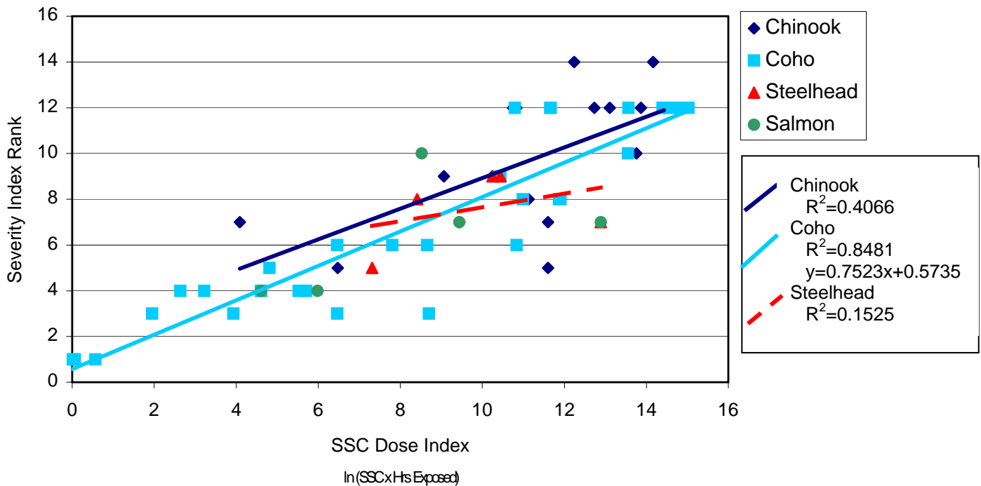
Figure 1 SSC Dose vs. Severity Index Rank for Chinook, Coho, and Steelhead (data from Newcombe & Jensen 1996)
