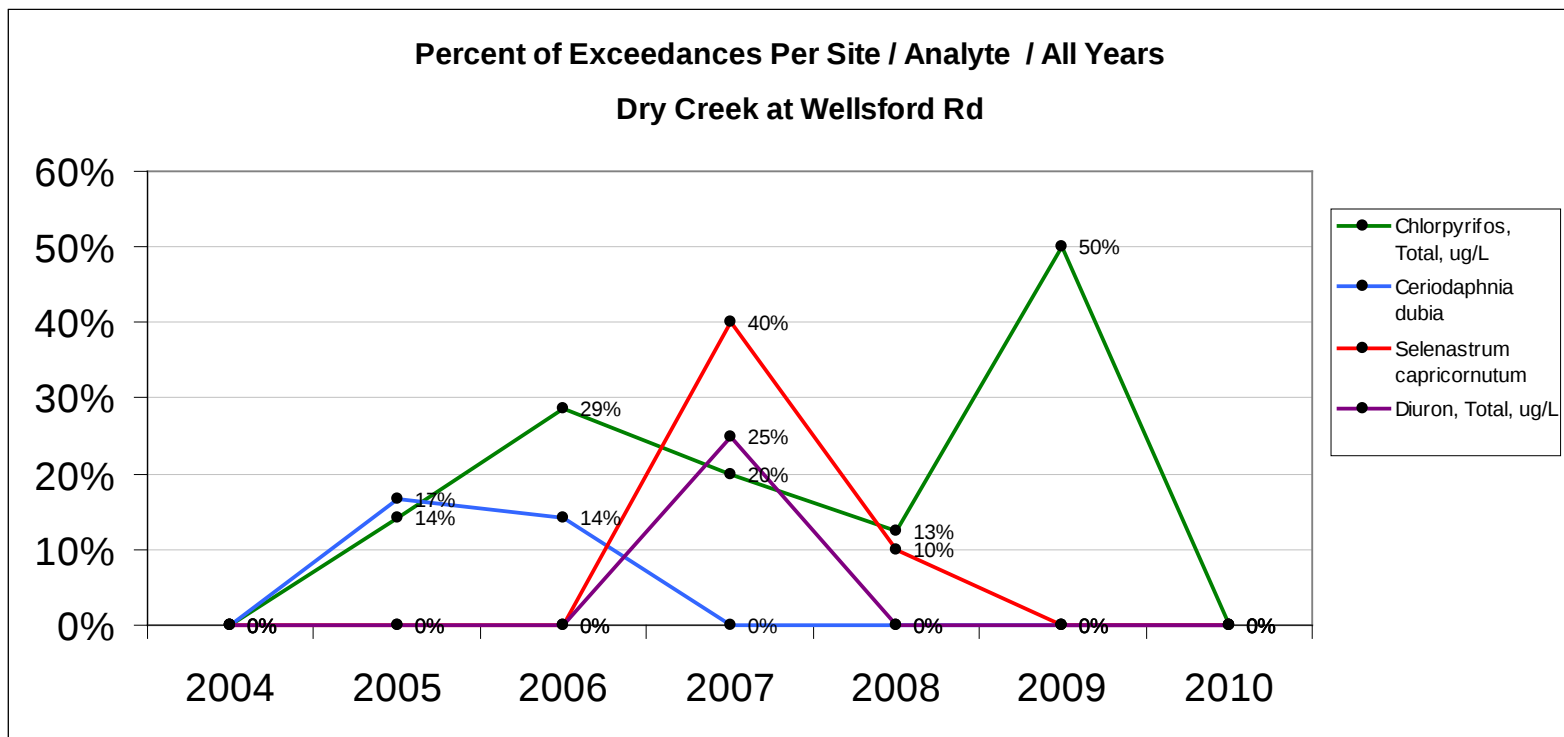
Figure 1. Percent of Exceedances Per Site / Analyte / All Year for Dry Creek at Wellsford Road
