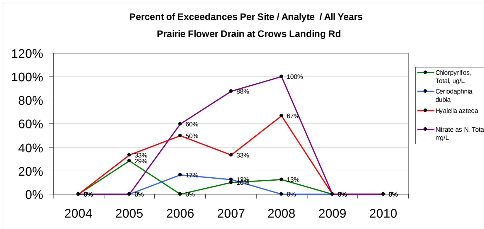
Figure 3. Percent of Exceedances Per Site / Analyte / All Year for Prairie Flower Drain at Crows Landing Road
