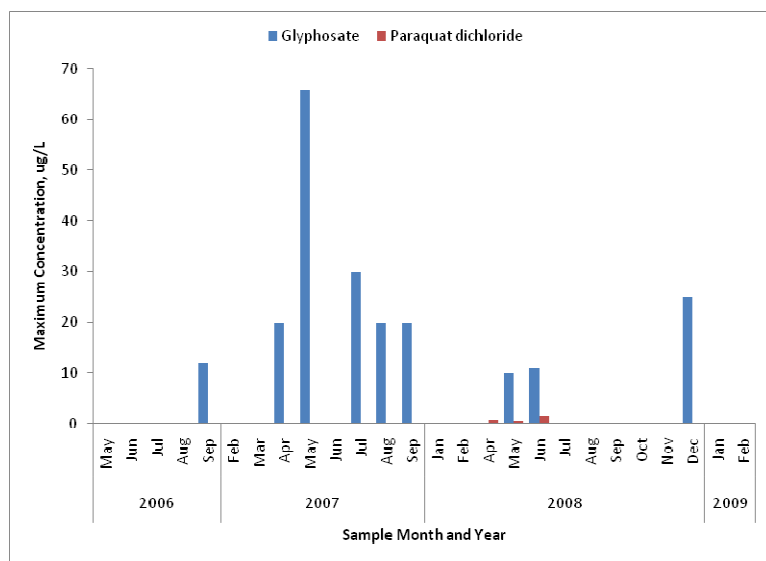
Figure 5. Maximum concentration of glyphosate and paraquat dichloride (2006-2009).
