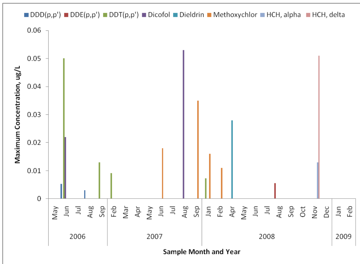
Figure 1. Organochlorines with one or more detection within the Coalition region from May 2006 through February 2009. The Coalition began monitoring for Group A pesticides in October 2008.
