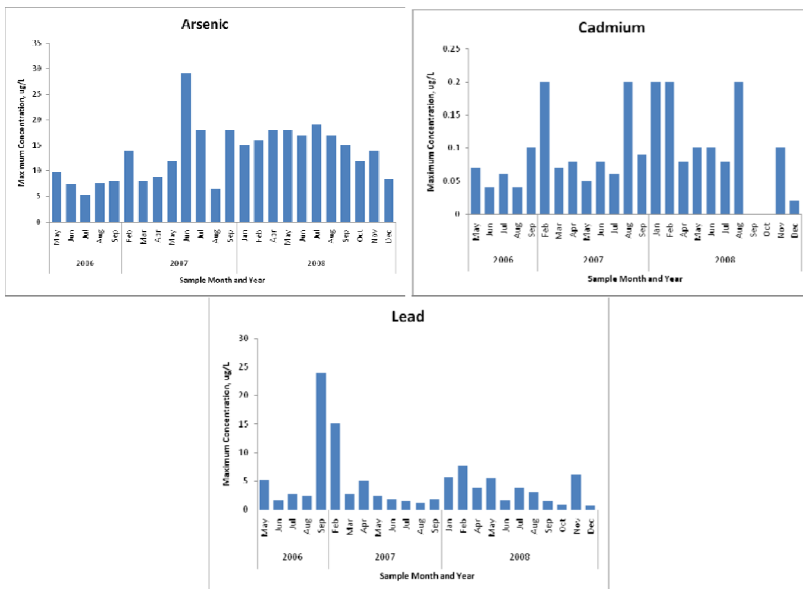
Figure 6. Maximum concentrations of arsenic, cadmium and lead (2006-2008).
