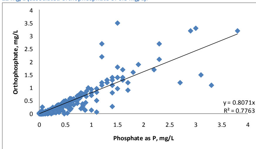
Figure 4. Linear regression of phosphate and orthophosphate (dissolved) omitting an outlier point with a phosphate value of 12 mg/L (associated orthophosphate of 6.8 mg/L).
