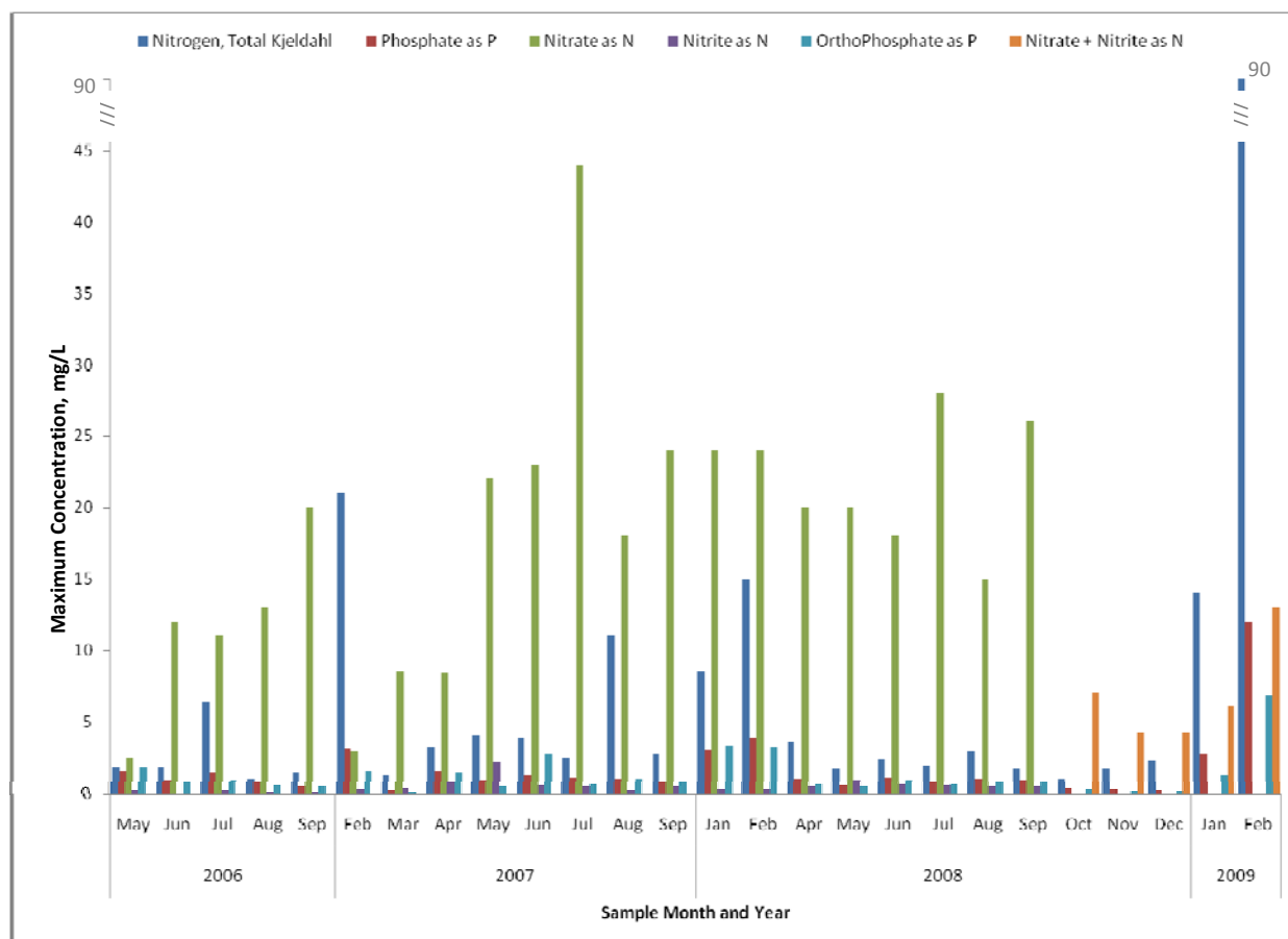
Figure 2. Maximum concentrations of nutrients (Total Kjeldahl Nitrogen, phosphate, nitrate, nitrite and orthophosphate) from 2006-2009.
