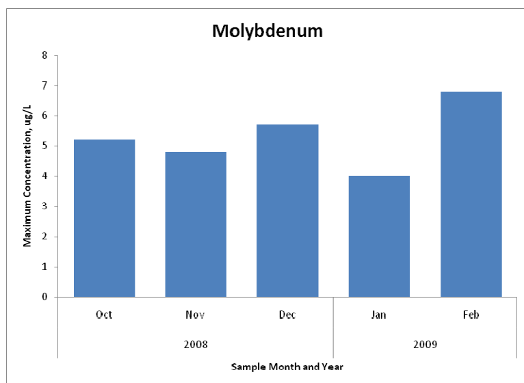
Figure 7. Maximum concentrations of molybdenum (2008-2009).
