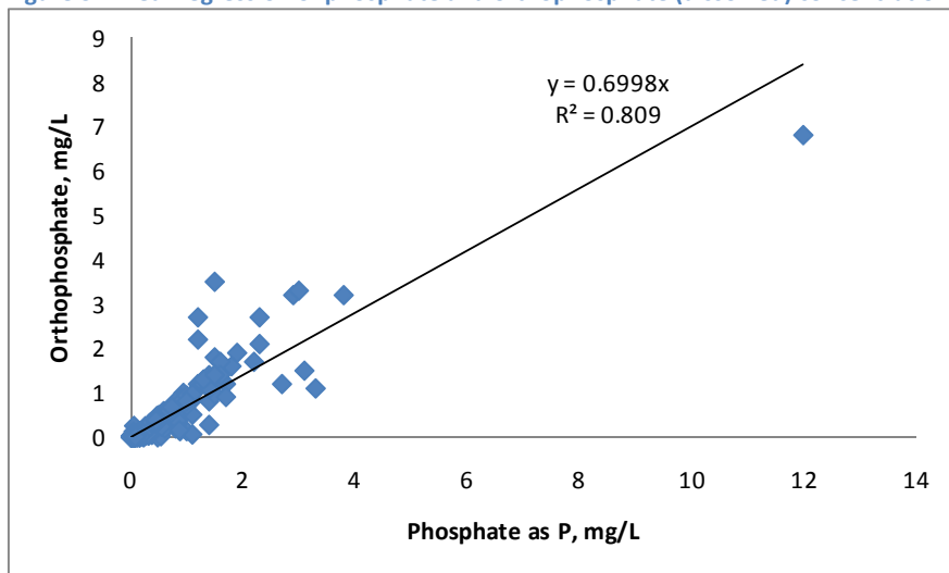
Figure 3. Linear regression of phosphate and orthophosphate (dissolved) concentrations (all results).
