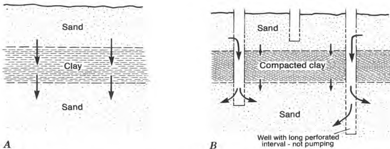
FIGURE 17.—Change in effective vertical conductance of Central Valley aquifer system due to development; size of arrows represents relative magnitude of flow. A, Predevelopment effective vertical conductance. B, Current effective vertical conductance.
