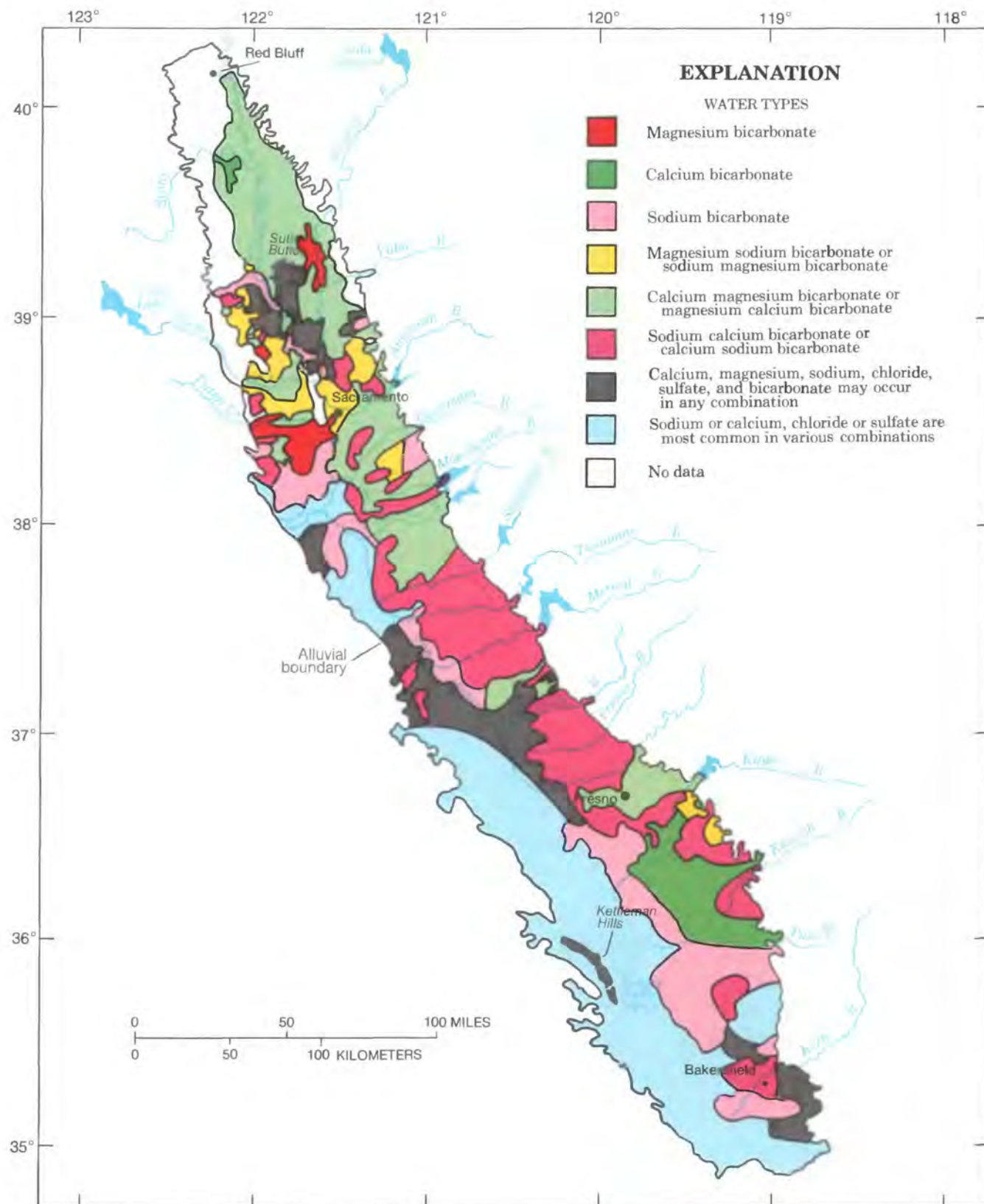
FIGURE 25. —Chemical types of ground water in the Central Valley. [Chemical types shown are approximated from maps and descriptions in the following reports: Davis and Poland, 1957; Wood and Davis, 1959; Wood and Dale, 1964; Dale and others, 1966; Croft and
