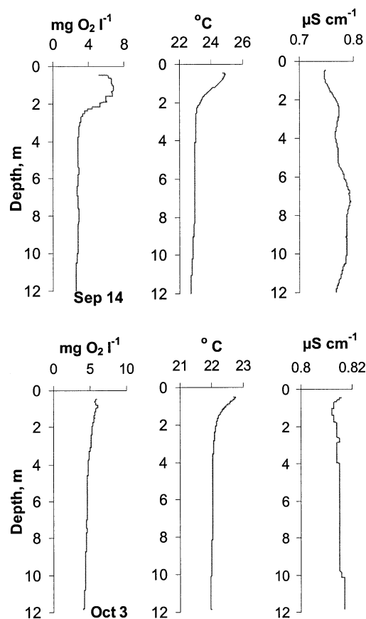
Fig. 6. Vertical profiles of dissolved oxygen concentration, water temperature and specific conductance at Rough and Ready Island in 2001.
