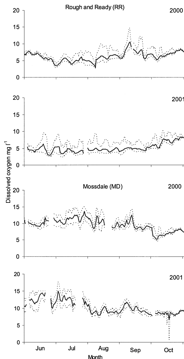
Fig. 3. Daily mean, maximum and minimum dissolved oxygen concentration in the Stockton Deep Water Channel (Channel) at Rough and Ready Island and Mossdale in 2000 and 2001.
