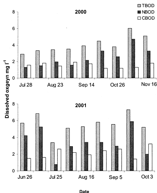
Fig. 8. Average total (TBOD), nitrogenous (NBOD), and carbonaceous (CBOD) oxygen demand determined from laboratory assays during 2000 and 2001.
