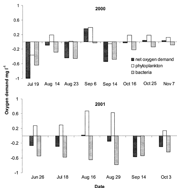
Fig. 7. Net, phytoplankton and bacterial oxygen demand in the Stockton Deep Water Channel in 2000 and 2001 based on in situ production rate measurements.
