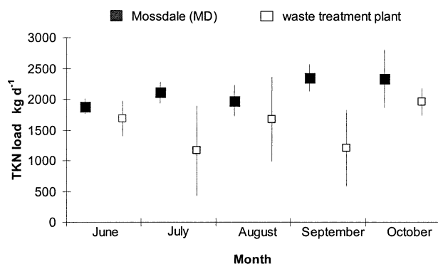
Fig. 9. Comparison of the average daily load of total Kjeldahl nitrogen into the Stockton Deep Water Channel from the Stockton Wastewater Treatment Plant and Mossdale (MD) upstream in 2001.
