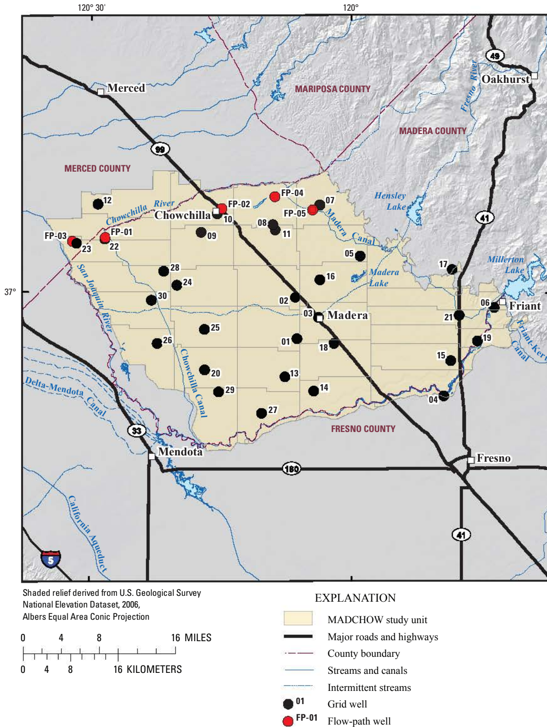
Figure 3. The Madera–Chowchilla Groundwater Ambient Monitoring and Assessment (GAMA) study unit showing the distribution of study area grid cells and the location of sampled grid wells and flow-path wells. Alphanumeric identification numbers for grid wells have the prefix “MADCHOW”; only the numeric portions are shown on the map. Alphanumeric identification numbers for flow-path wells have the prefix “MADCHOWFP”; only “FP” and the numeric portions are shown on the map.
