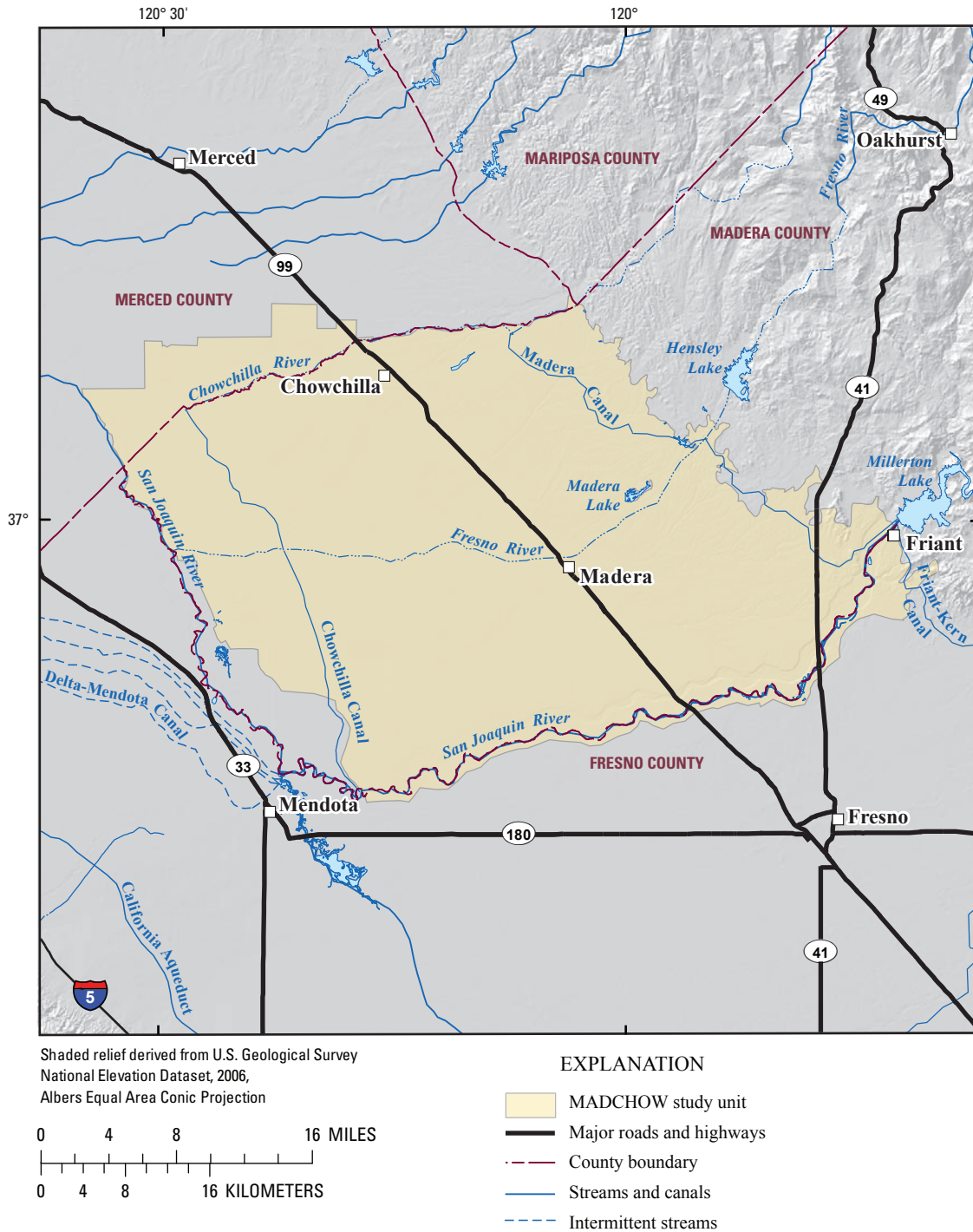
Figure 2. The Madera–Chowchilla Groundwater Ambient Monitoring and Assessment (GAMA) study unit showing locations of major cities and major hydrologic features.
