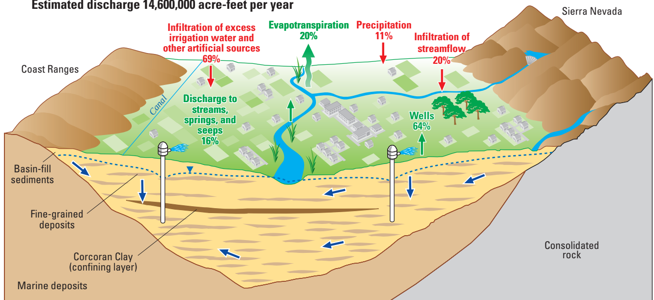
Figure 2. Generalized diagrams for the Central Valley, California, showing the basin-fill deposits and components of the groundwater system under (A) predevelopment and (B) modern conditions.
