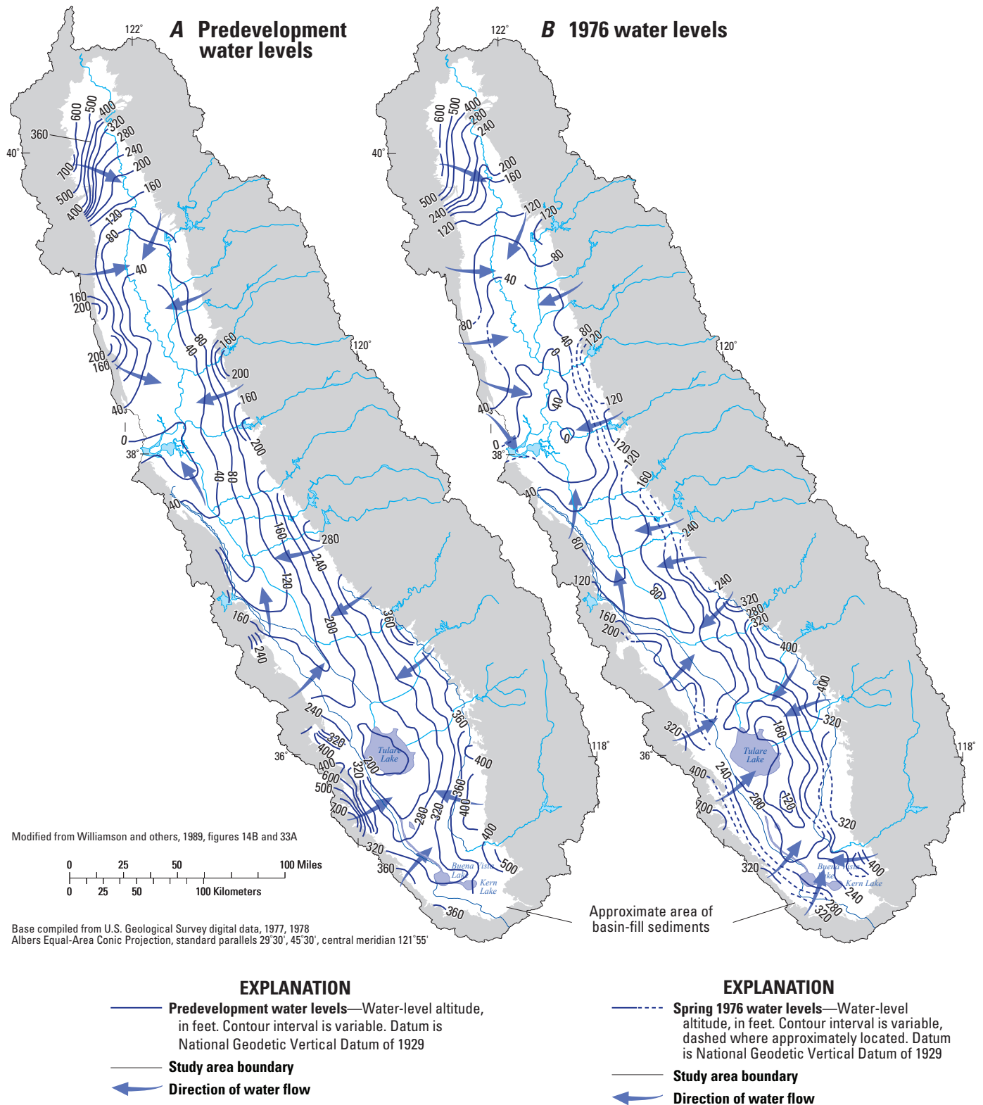
Figure 3. Groundwater levels in the unconfined part of the aquifer system in the Central Valley, California (A) estimated for predevelopment conditions, and (B) in 1976.
