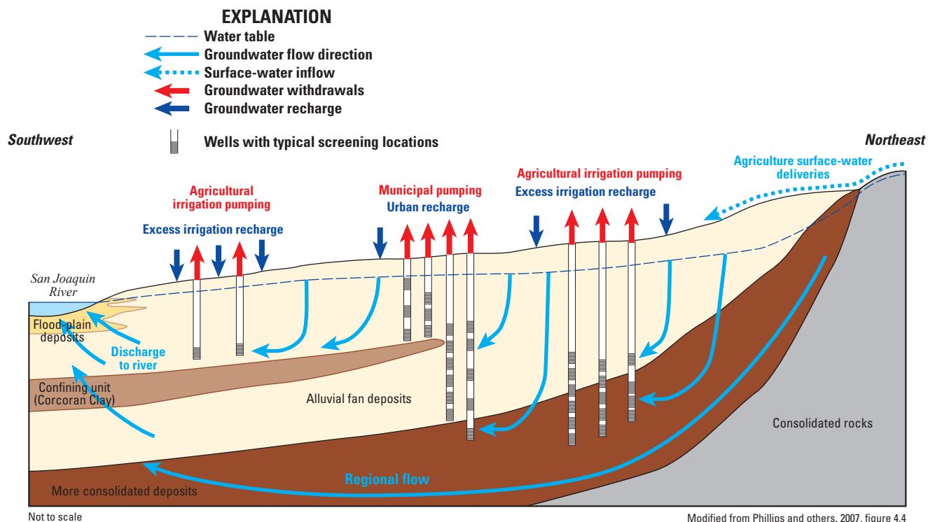
Figure 4. Conceptual diagram showing effects of pumping and irrigation on vertical groundwater flow, and natural discharge areas near Modesto, California.
