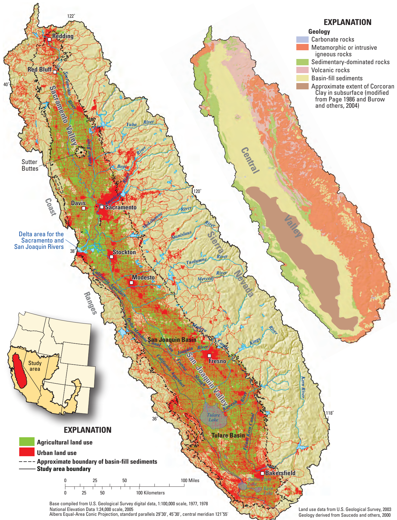
Figure 1. Physiography, land use, and generalized geology of the Central Valley, California.
