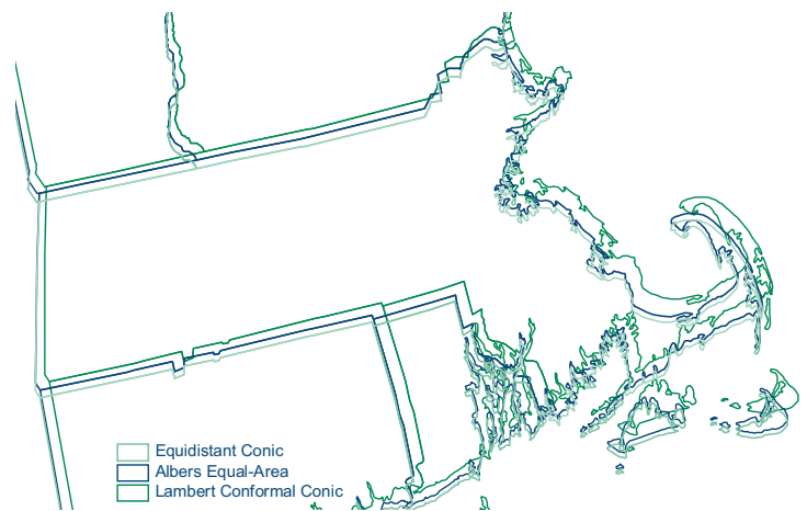
Figure 5-3. Example Map Projections
