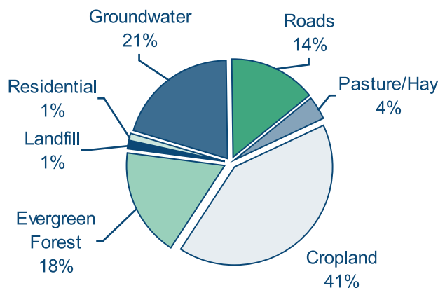
Figure 8-7. Total Sediment Load and Percentages Associated with Each Source
