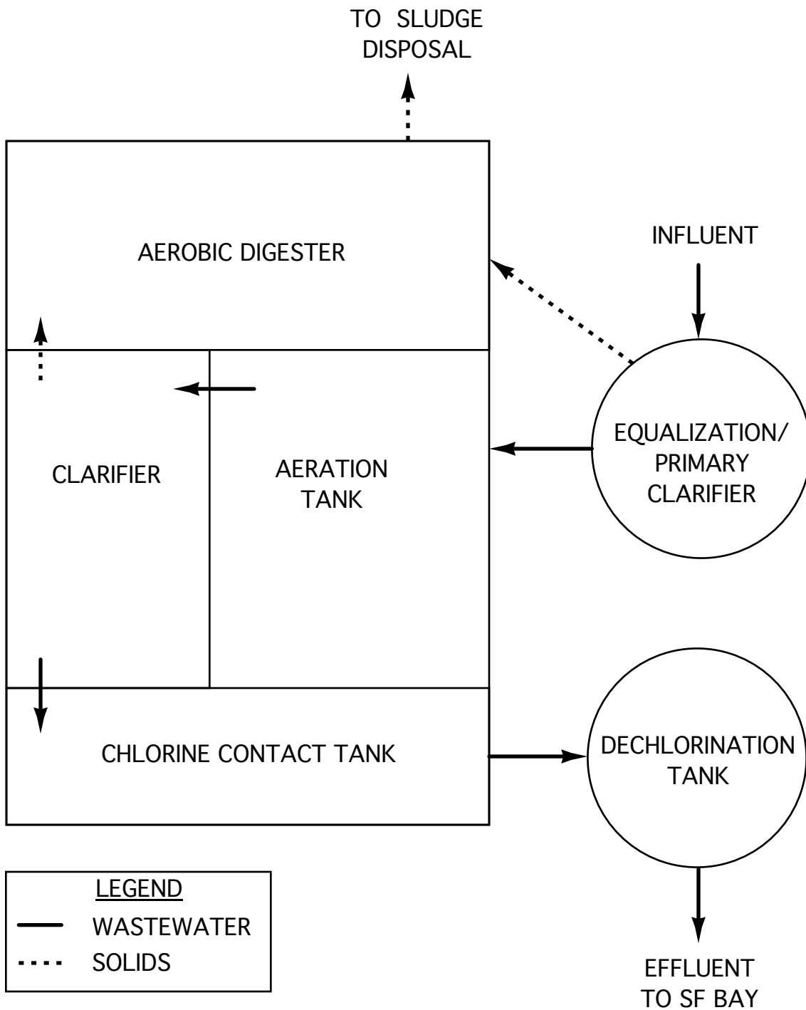
Sanitary District No. 5 of Marin County Paradise Cove WWTP Process Schematic
