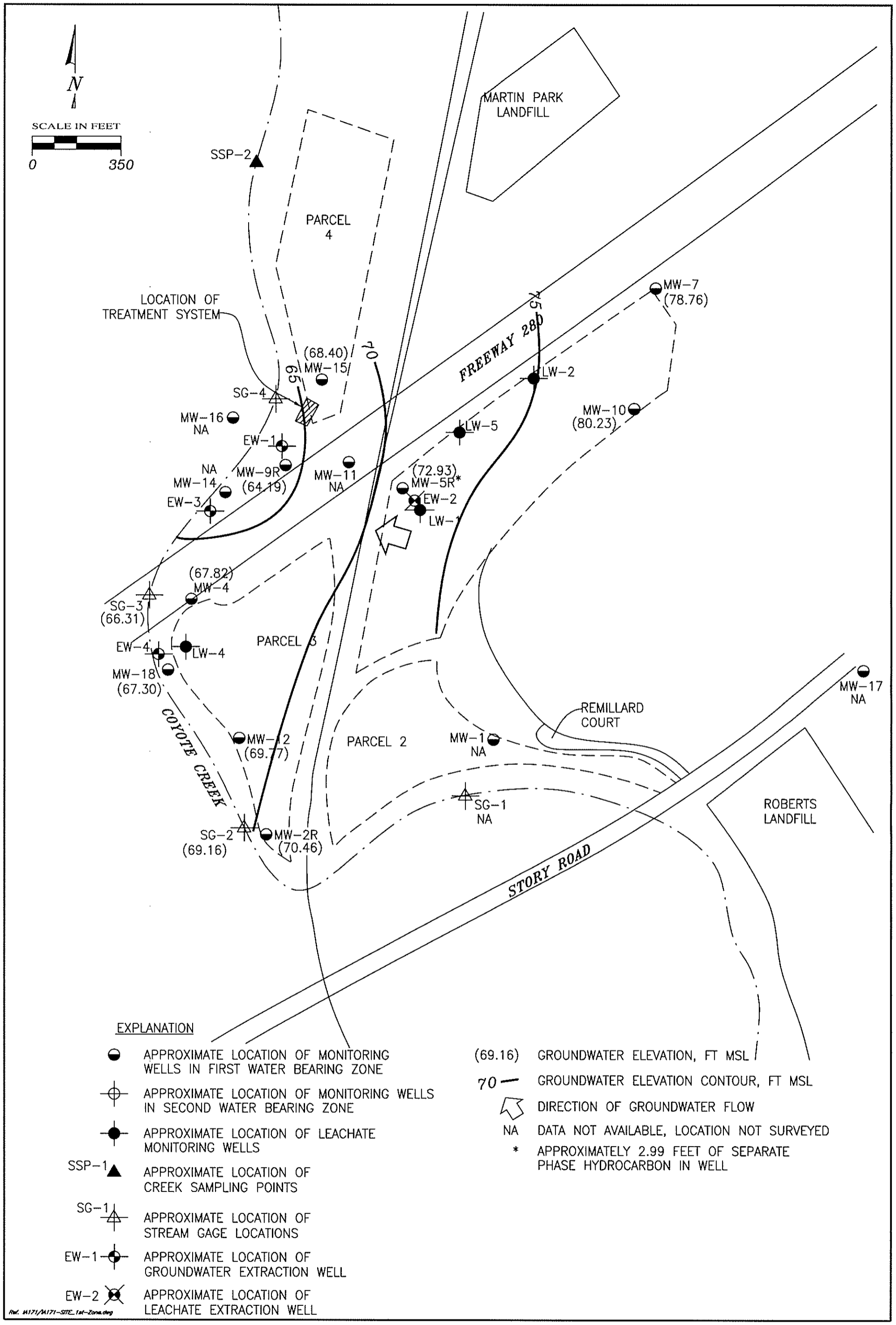
GROUNDWATER ELEVATION CONTOUR MAP A-ZONE SEPTEMBER 27, 2005 STORY ROAD LANDFILL San Jose, California
