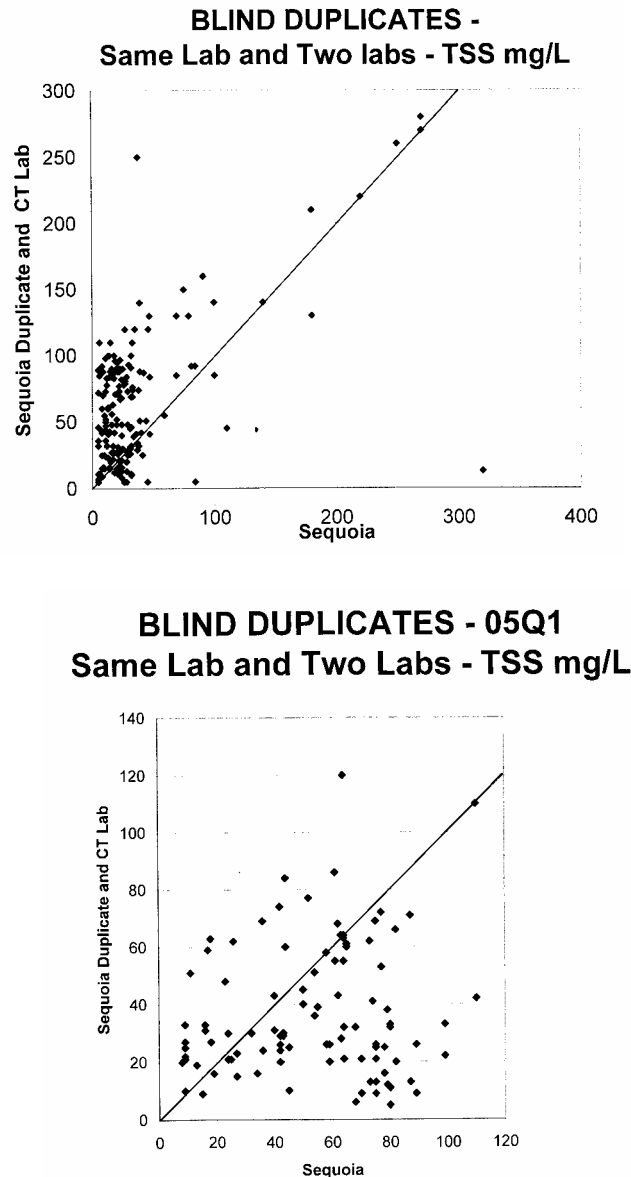
Figure 3. Blind duplicate samples from the second half of the year 2004 (upper) and first quarter 2005 (lower). In the upper plot, samples are from Oakland Yard and Marina Vista Yard, and include both discharge and internal process samples. In the lower plot, samples are Oakland effluent. The spread of
