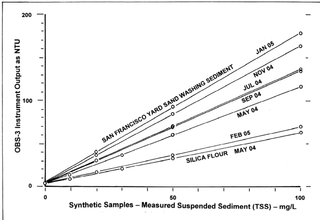
Figure 6. Relation Of OBS Instrument Output Versus Synthetic Suspended Particle Concentration for Various Samples. Most points represent repeated runs that plot in the same place, indicating very good precision. The output is very close to linear for each sample, although the curves actually bend slightly downward. The May 2004 San Francisco Yard sample was collected from the bottom of the final settling pond, while all subsequent samples were collected by settling sediment from the liquid entering the pond. The difference between the May 2004 and Feb 2005 Silica Flour samples suggests minor instrument drift, whereas most of the difference in the San Francisco Yard samples is interpreted to be due to differences in material properties.
