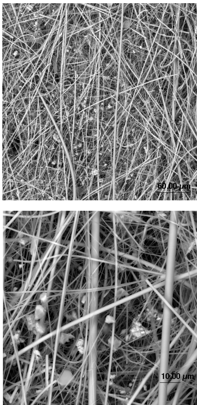
Figure 11. Scanning electron microscope photo of TSS filter used for sand yard discharge water, at two scales.
