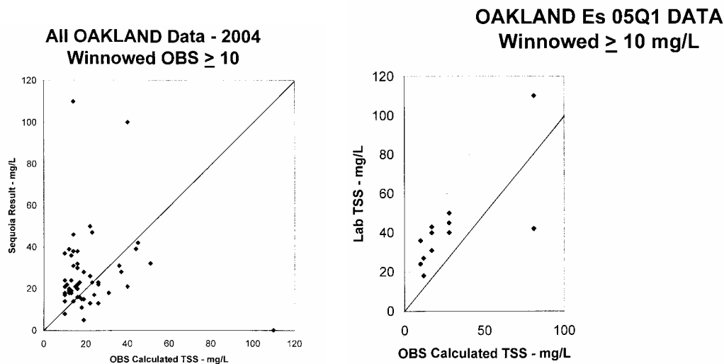
Figure 8. Comparison of Results: OBS and EPA Method 160.2 for Oakland Yard 2004 (Left Plot) and First Quarter 2005 (Right Plot) – OBS \geq 10 mg/L.
