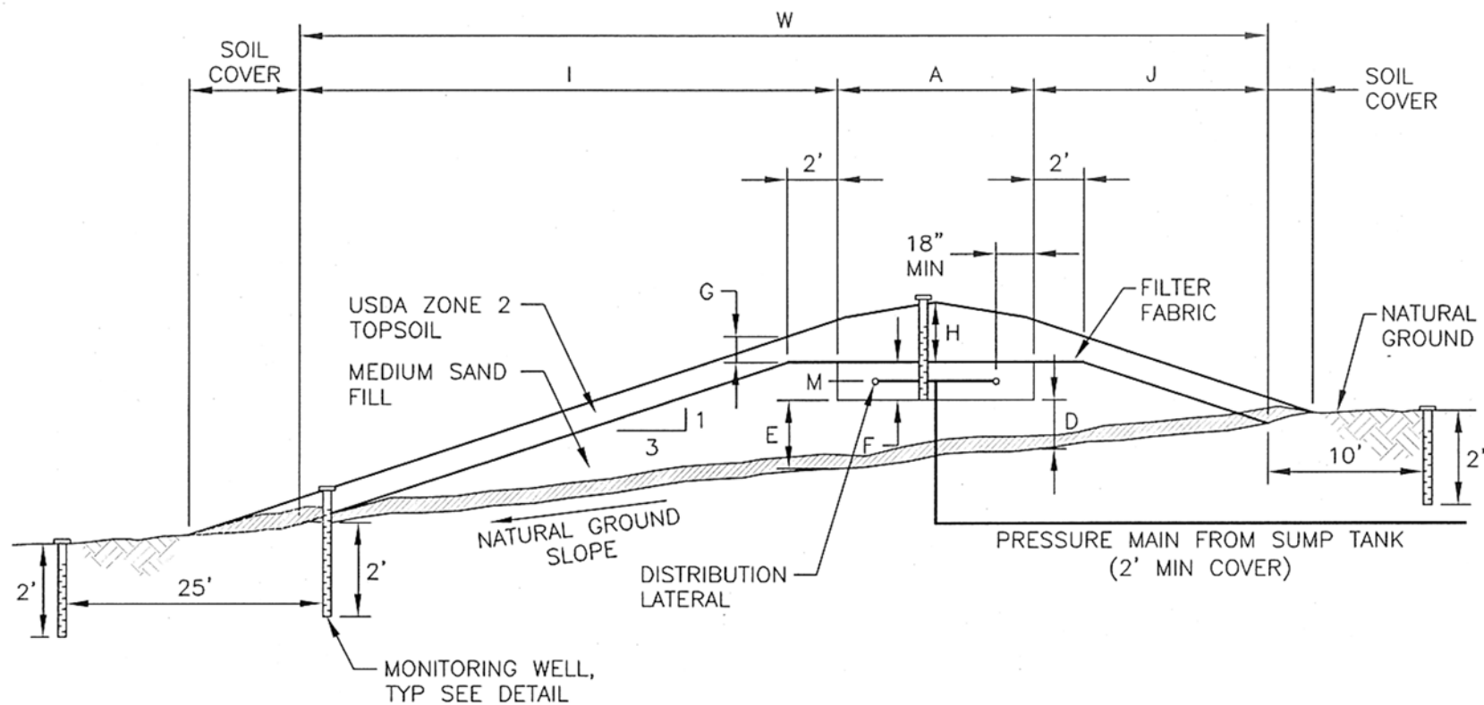
CROSS SECTION DIMENSIONS (SLOPING SITE)
