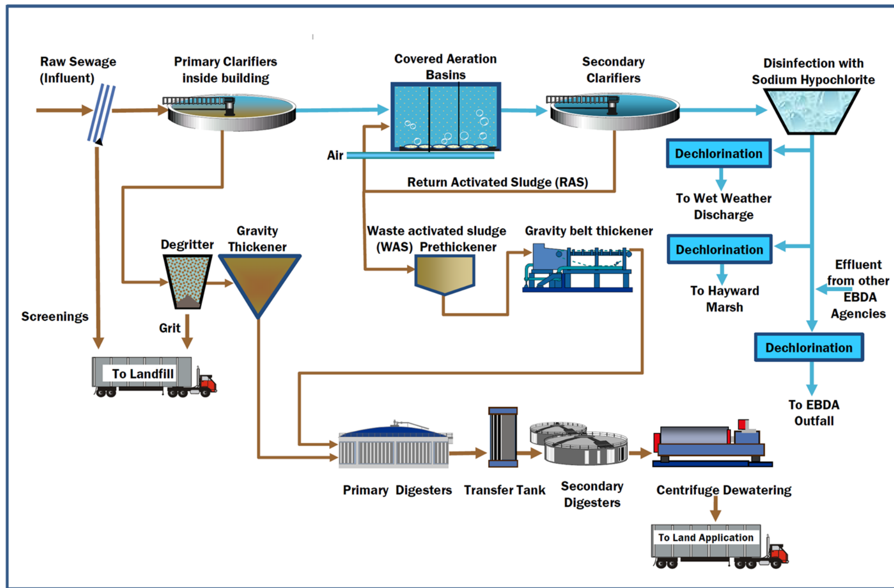
Figure C-2A. Treatment Plant Schematic (With Hayward Marsh)
