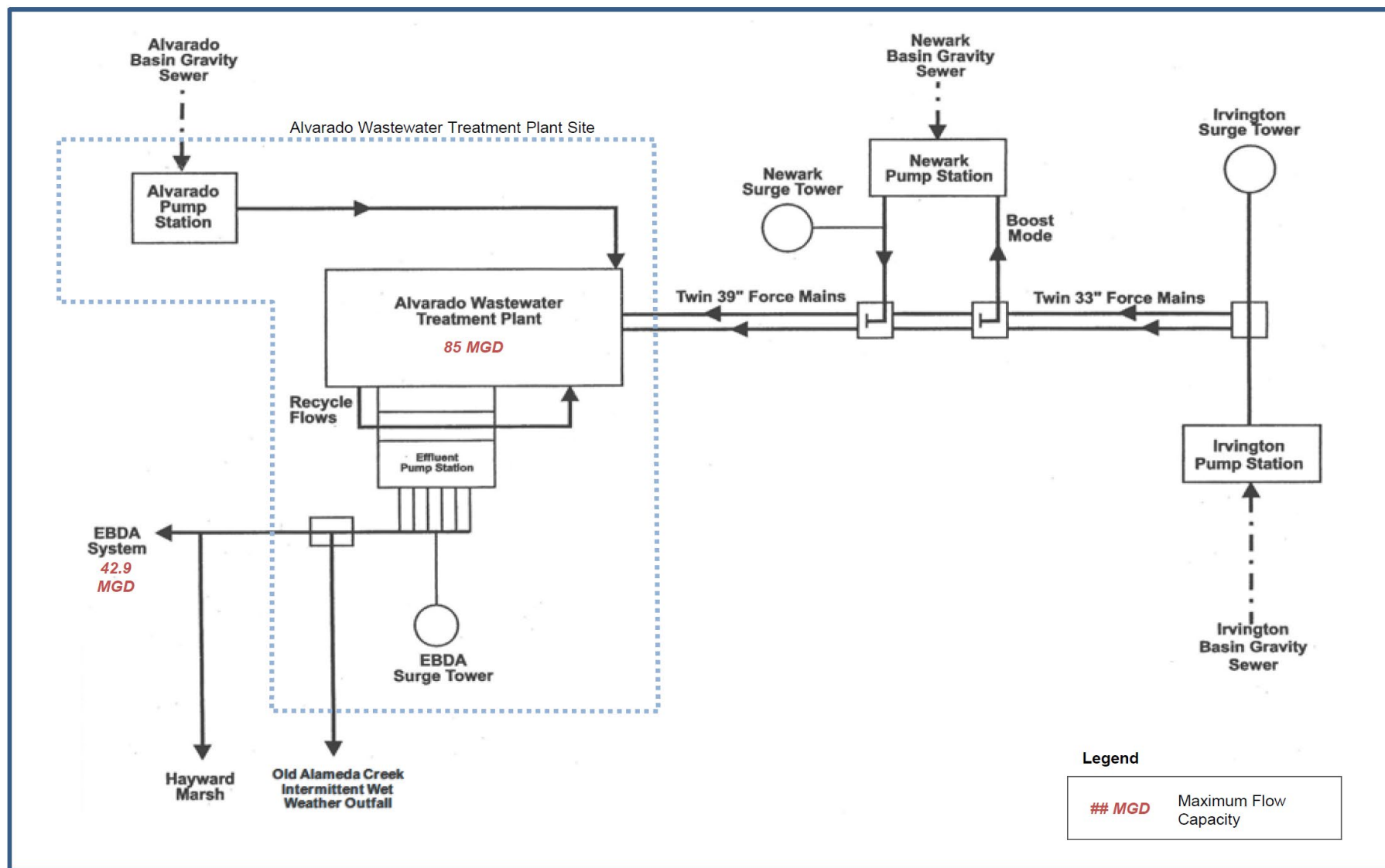
Figure C-1A. Influent and Effluent Transport System Schematic (With Hayward Marsh)
