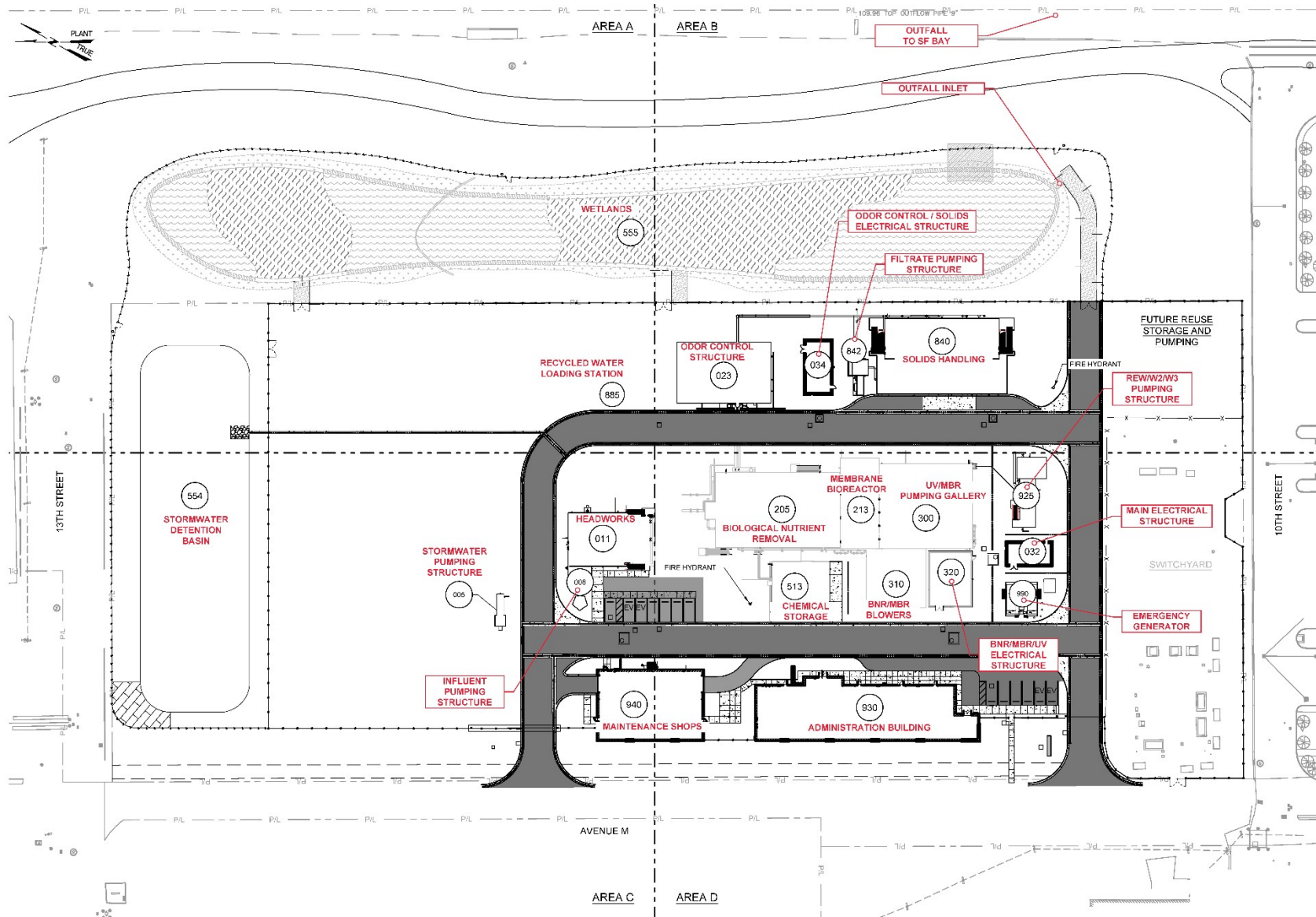
Figure B-3. Facility Layout
