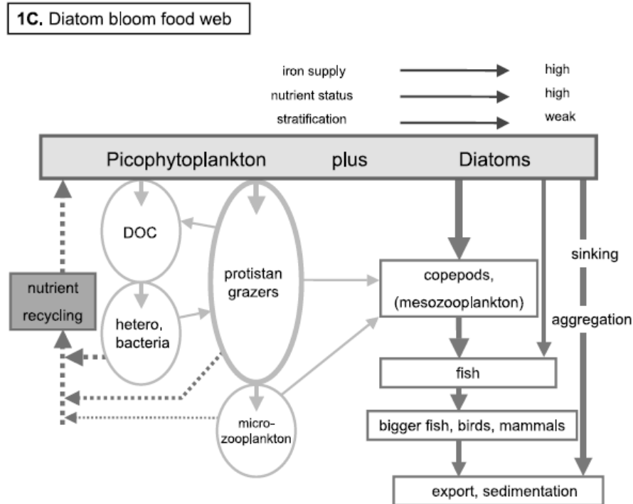
Figure 3.6. Example of a marine food web showing the complex pico-phytoplankton and diatom food web structure in diatom-dominated blooms. For simplicity, the regeneration paths are shown only on the left side of the figure (Source: Barber and Hiscock 2006).
