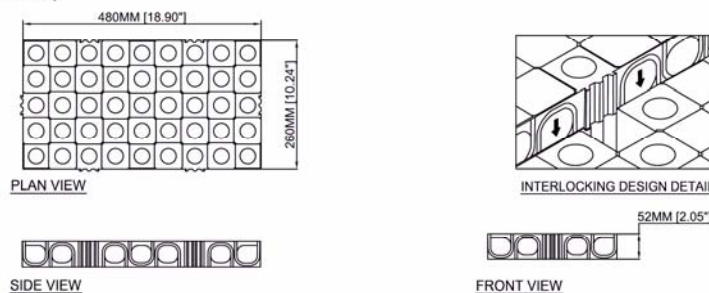
ATLANTIS DRAINAGE CELL (52MM CELL) OR EQUIVALENT
