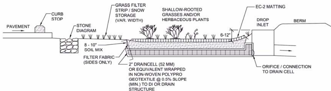
FIGURE 4: DESIGN CONCEPT #2 HIGH WATER TABLE OR SHALLOW TO BEDROCK CONCEPT: SHALLOW SYSTEM WITH DRAIN CELL DETAIL
