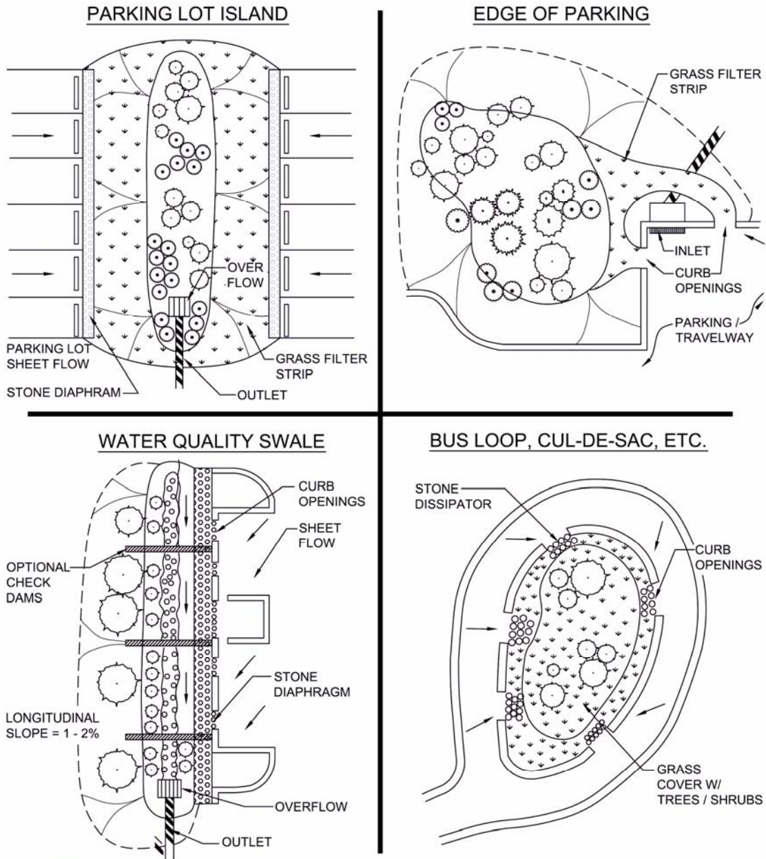
FIGURE 1: BIORETENTION APPLICATIONS - COMMERCIAL, INSTITUTIONAL DETAIL NTS
