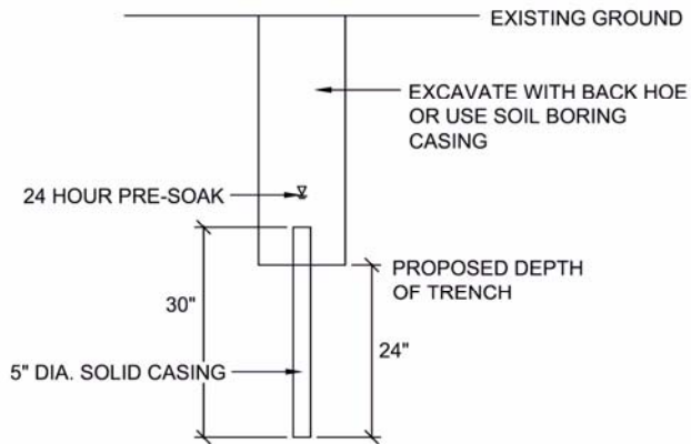
FIGURE 11: INFILTRATION TESTING DETAIL
