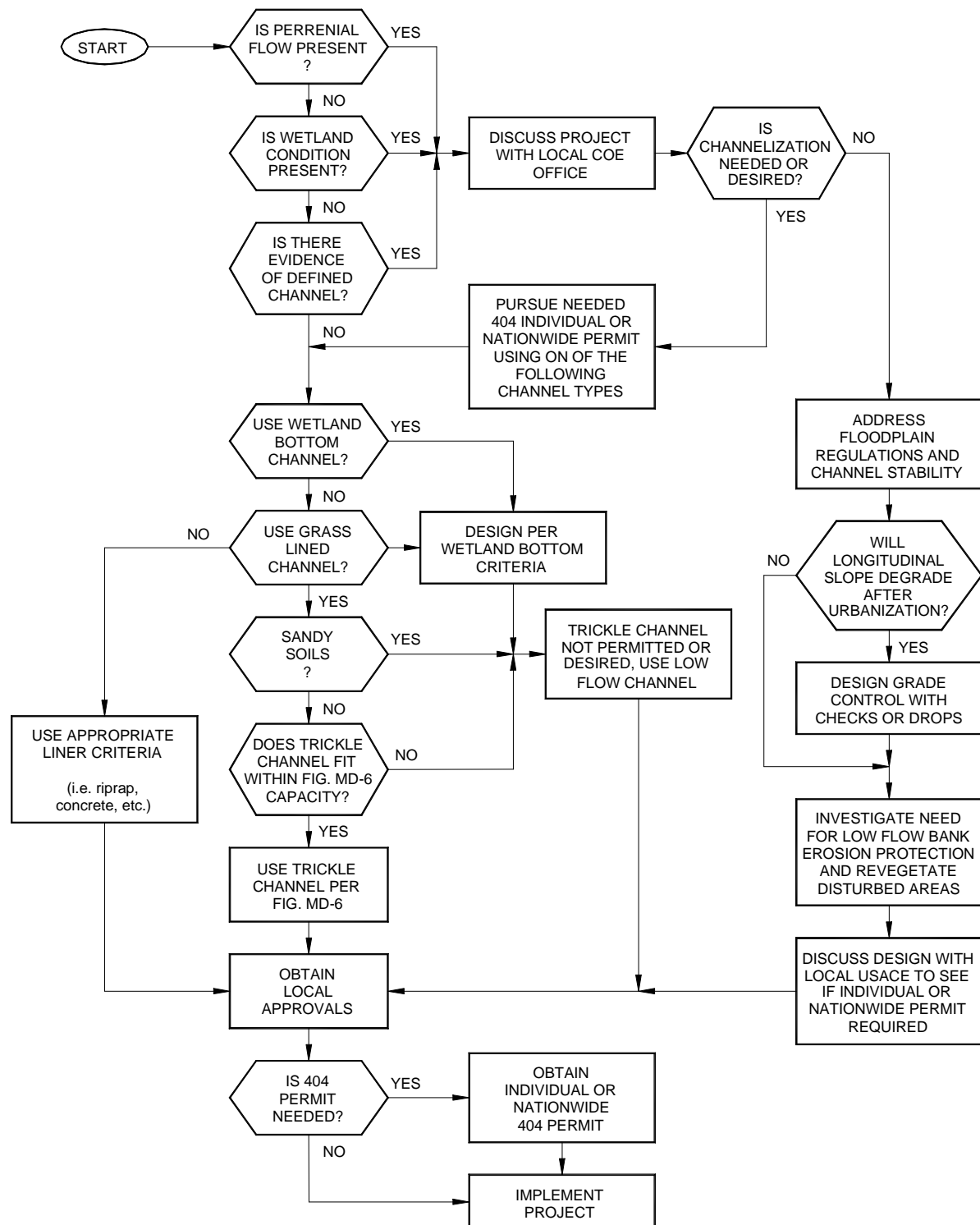
Figure MD-4—Flow Chart for Selecting Channel Type and Assessing Need for 404 Permit
