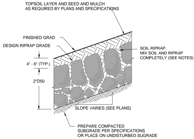
TYPICAL SECTION - SOIL RIPRAP WITH MULCH
