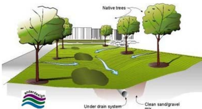
Fig. 1: Bio-swale schematic Courtesy Pierce County, /WSU Extension
