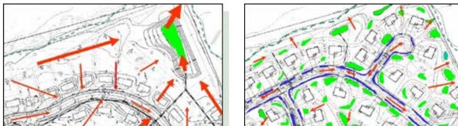
Figs. 2-3, Left to right : Conventional and LID site design comparison Courtesy PGDER
