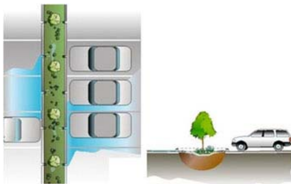
Fig. 19: Bio-retention cell schematic Courtesy Pierce County, Washington and AHBL, Inc.
