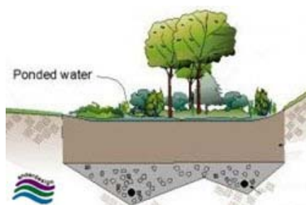
Fig. 9: Open space is used for storm water control via a Bio-retention Cell Courtesy Pierce County, WA/WSU Extension
