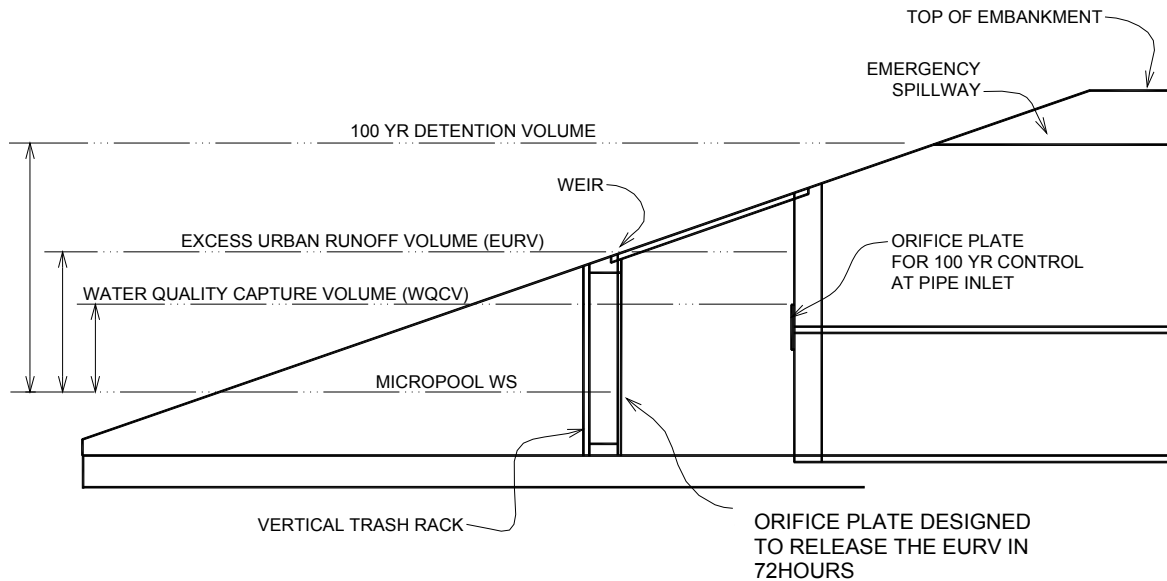
EXAMPLE OUTLET STRUCTURE
