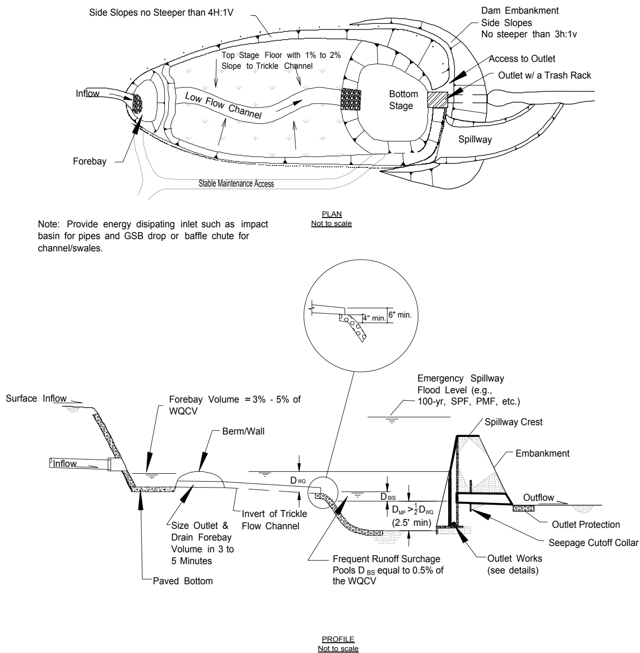
Figure SO-6—Plan and Profile of an Extended Detention Basin in a Flood Control Detention Basin
