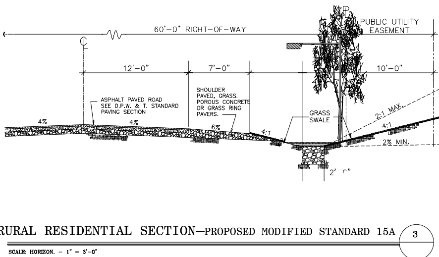
Figure 2-10. Typical road sections (Prince George's County, MD, 1997)
