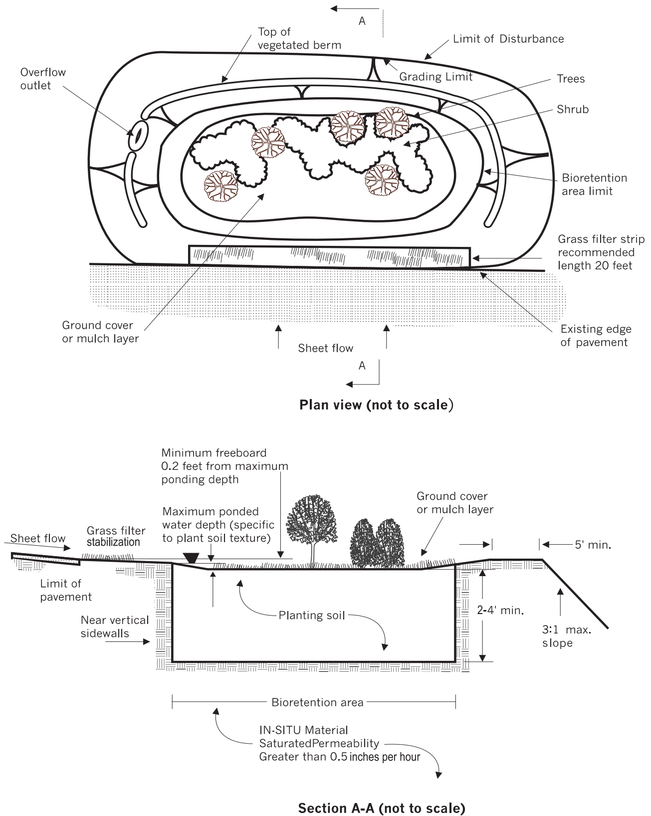
Figure 4-3. Typical bioretention facility
