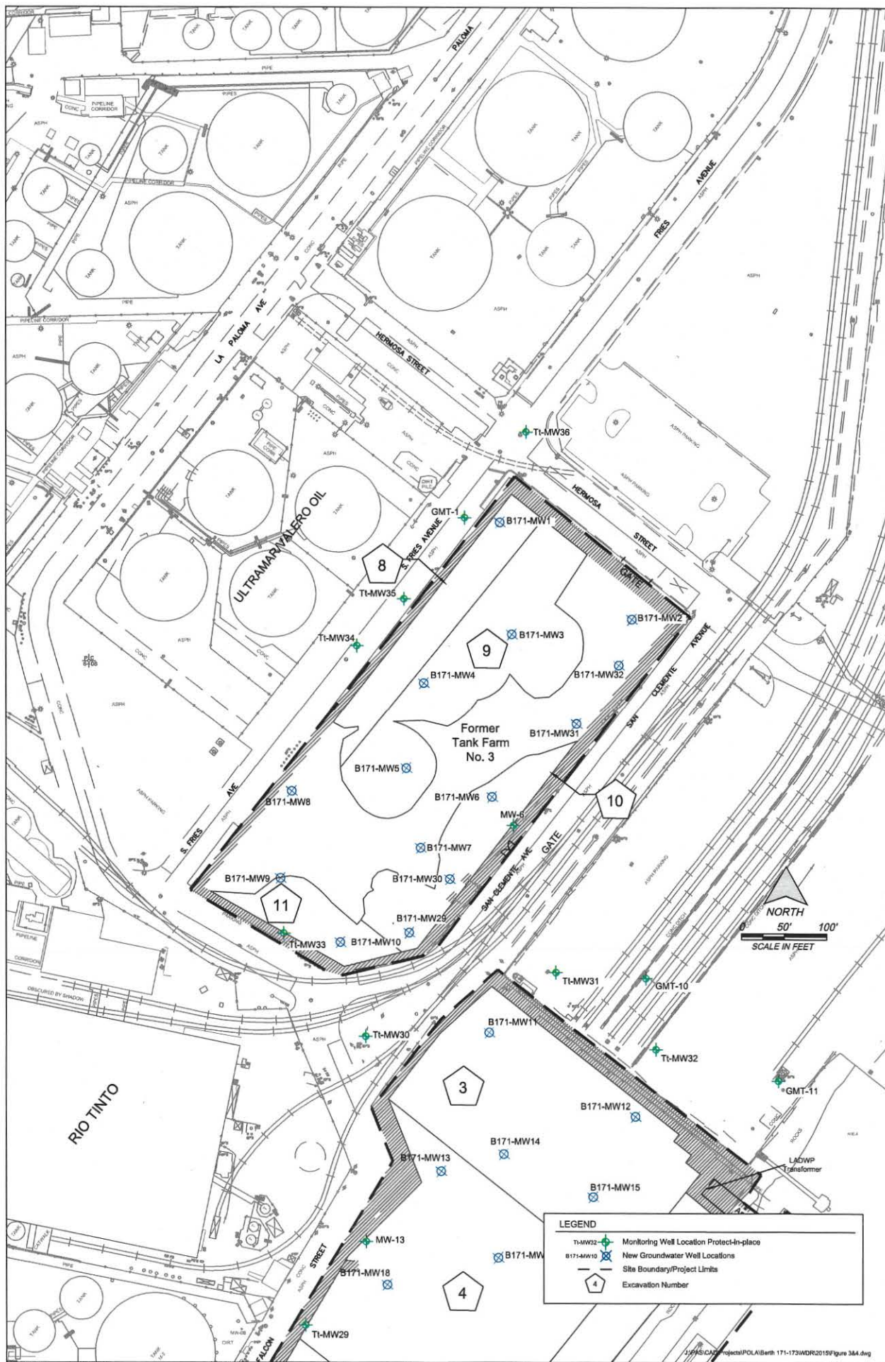
FIGURE 3 TANK FARM NO. 3 PROPOSED GROUNDWATER MONITORING WELLS WITH PROTECT-IN-PLACE AND EXCAVATION AREAS
