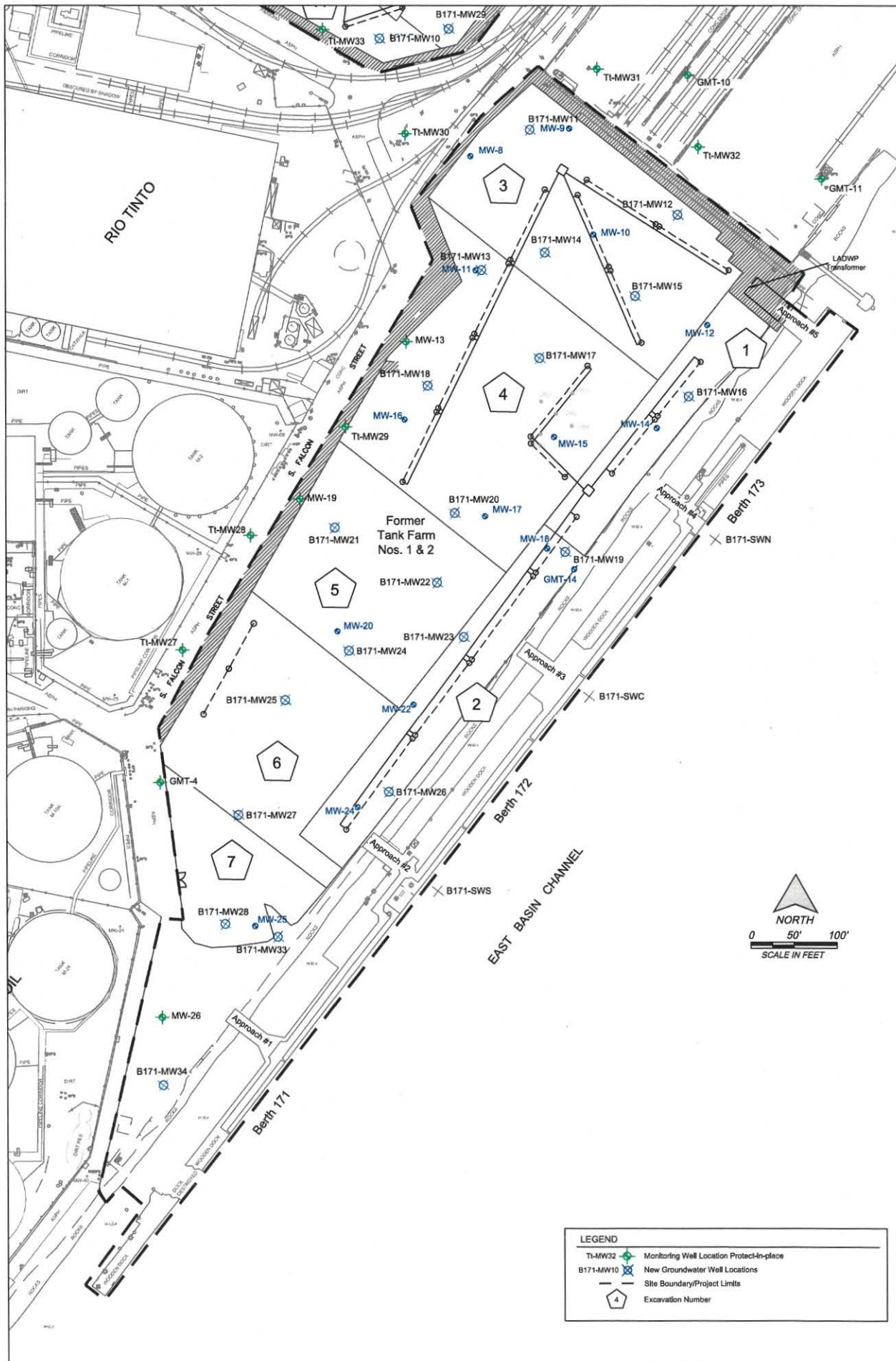
FIGURE 2 TANK FARM NOS. 1 & 2 PROPOSED GROUNDWATER MONITORING WELLS WITH PROTECT-IN-PLACE AND EXCAVATION AREAS
