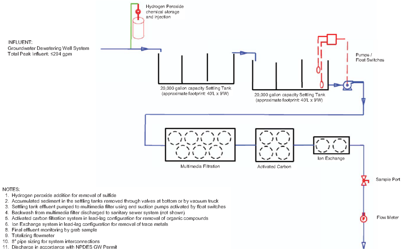
Figure 3. Treatment Process at 5150 Wilshire Boulevard
