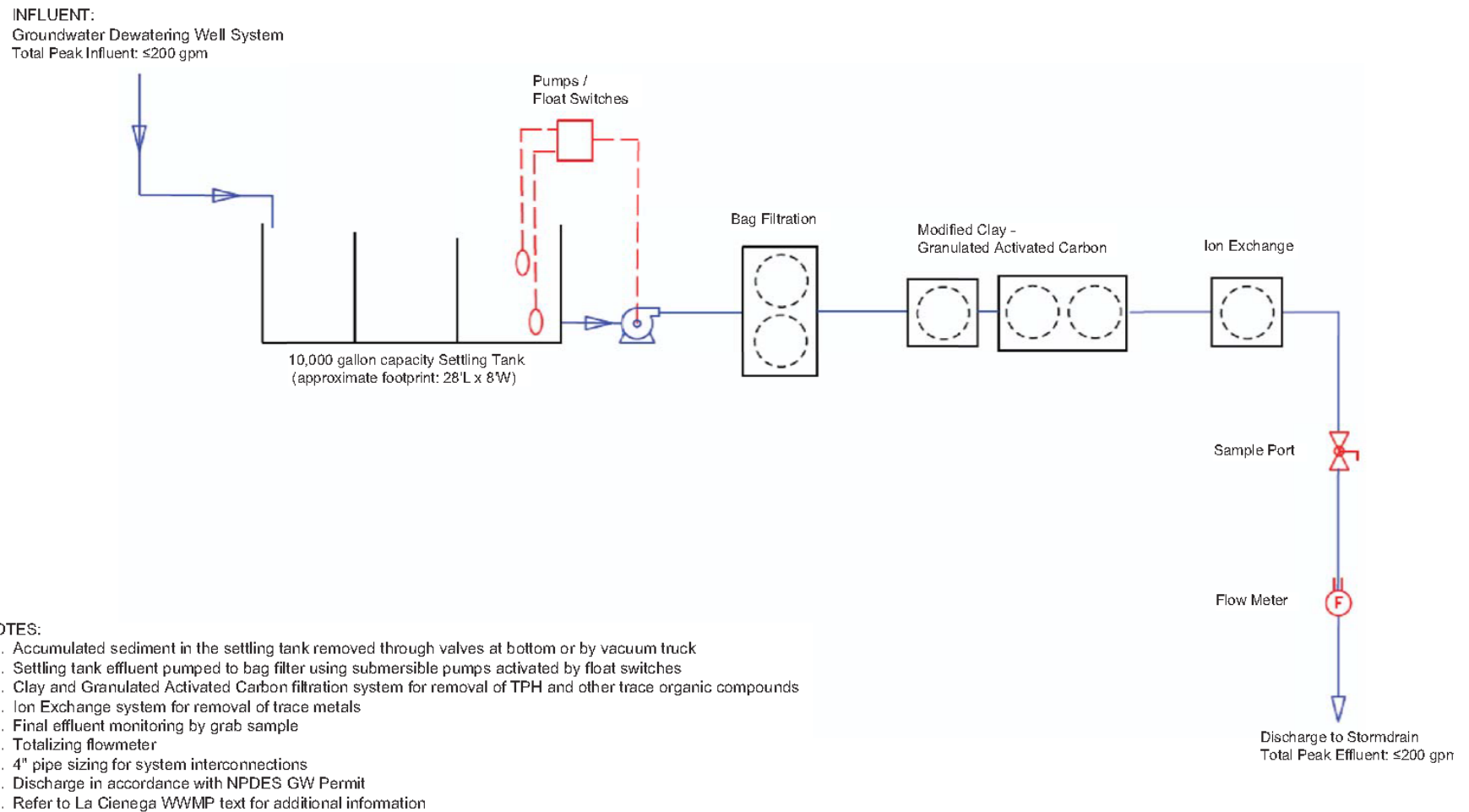
Figure 4. Treatment Process at 8350 Wilshire Boulevard
