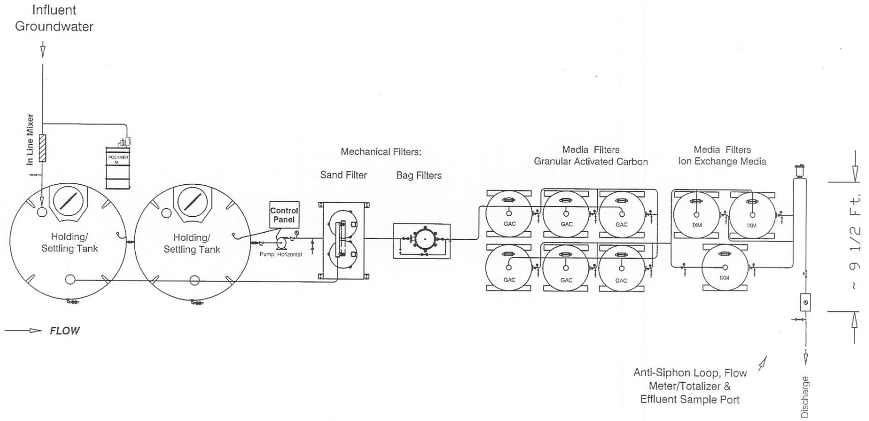
Figure 2. Treatment Process
