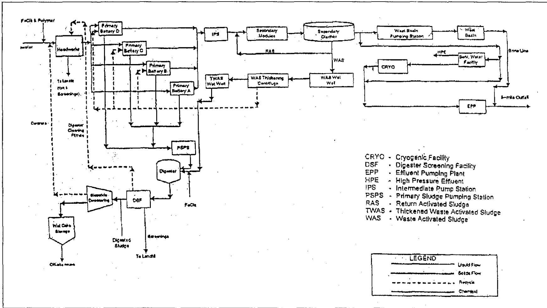
Figure P3 – Schematic of Wastewater Flow at Hyperion Treatment Plant
