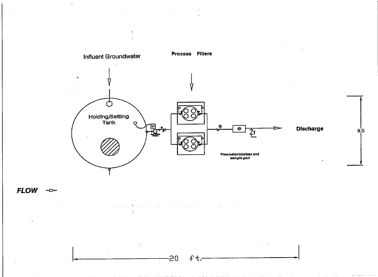
Figure 2. Treatment Schematics
