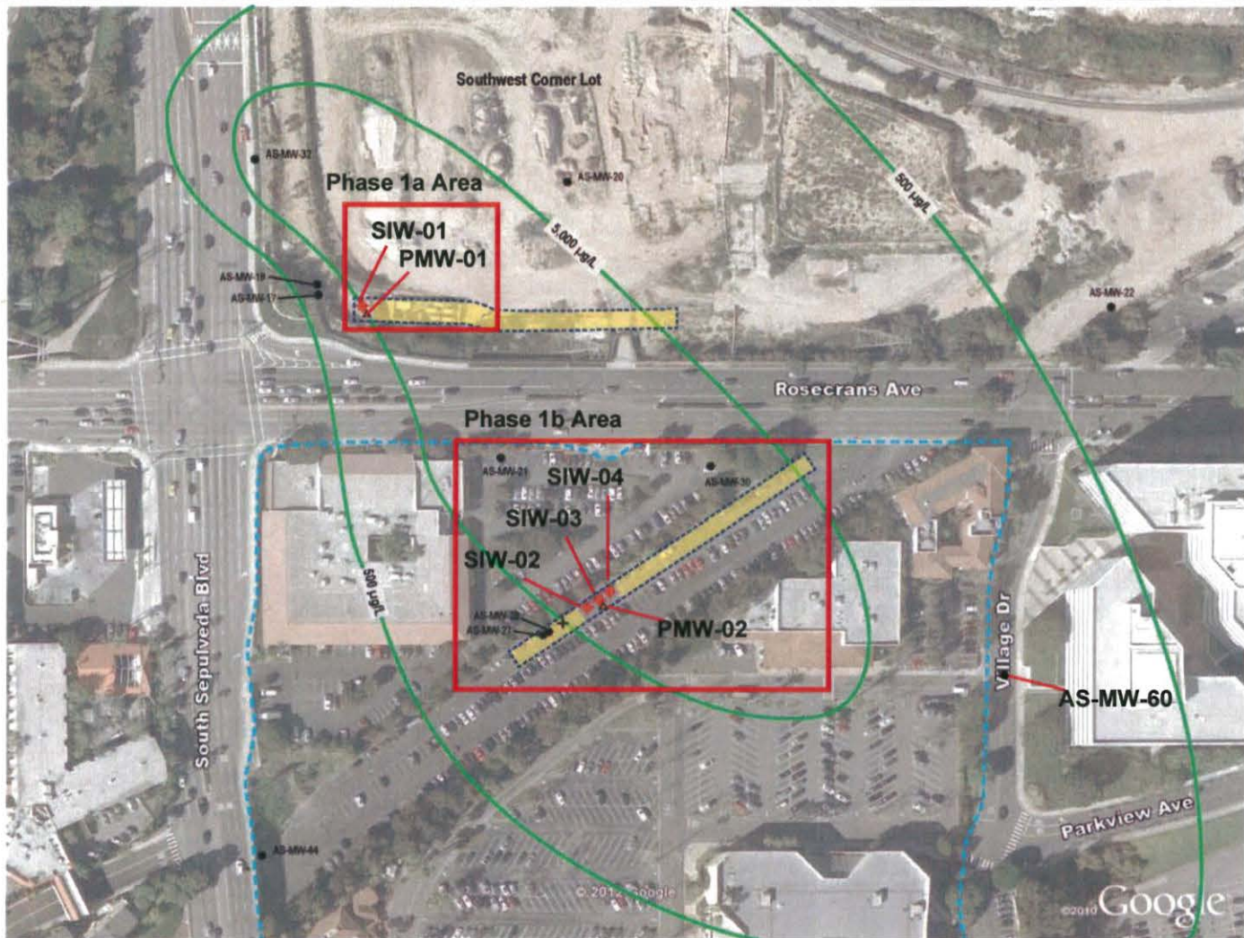
FIGURE 1 Proposed Conceptual Layout for Phased ERD Wells
