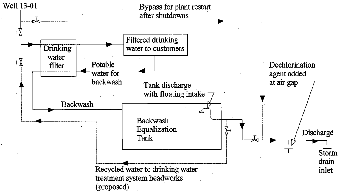
Figure 2. Treatment Schematic
