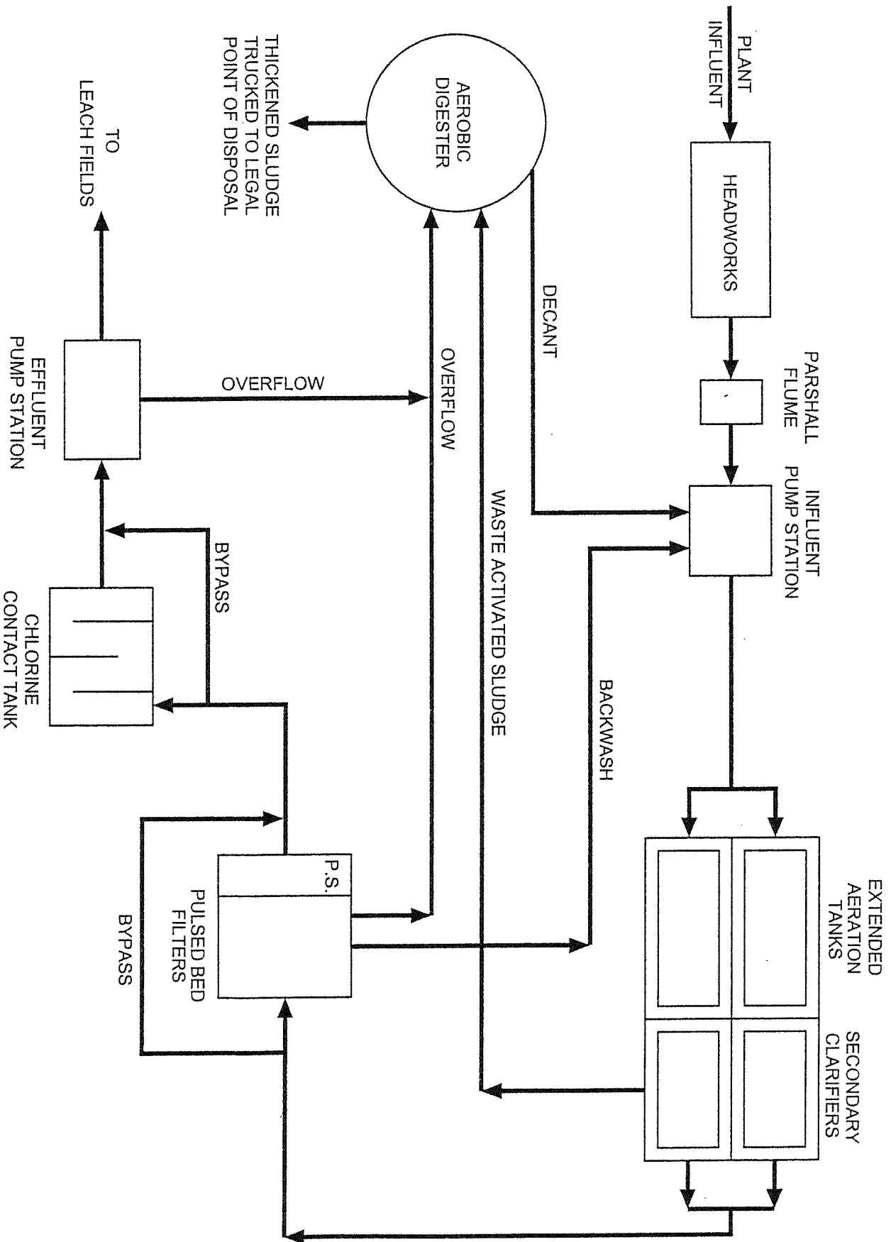
FIGURE 3. TRANCAS WPCP FLOW CHART
