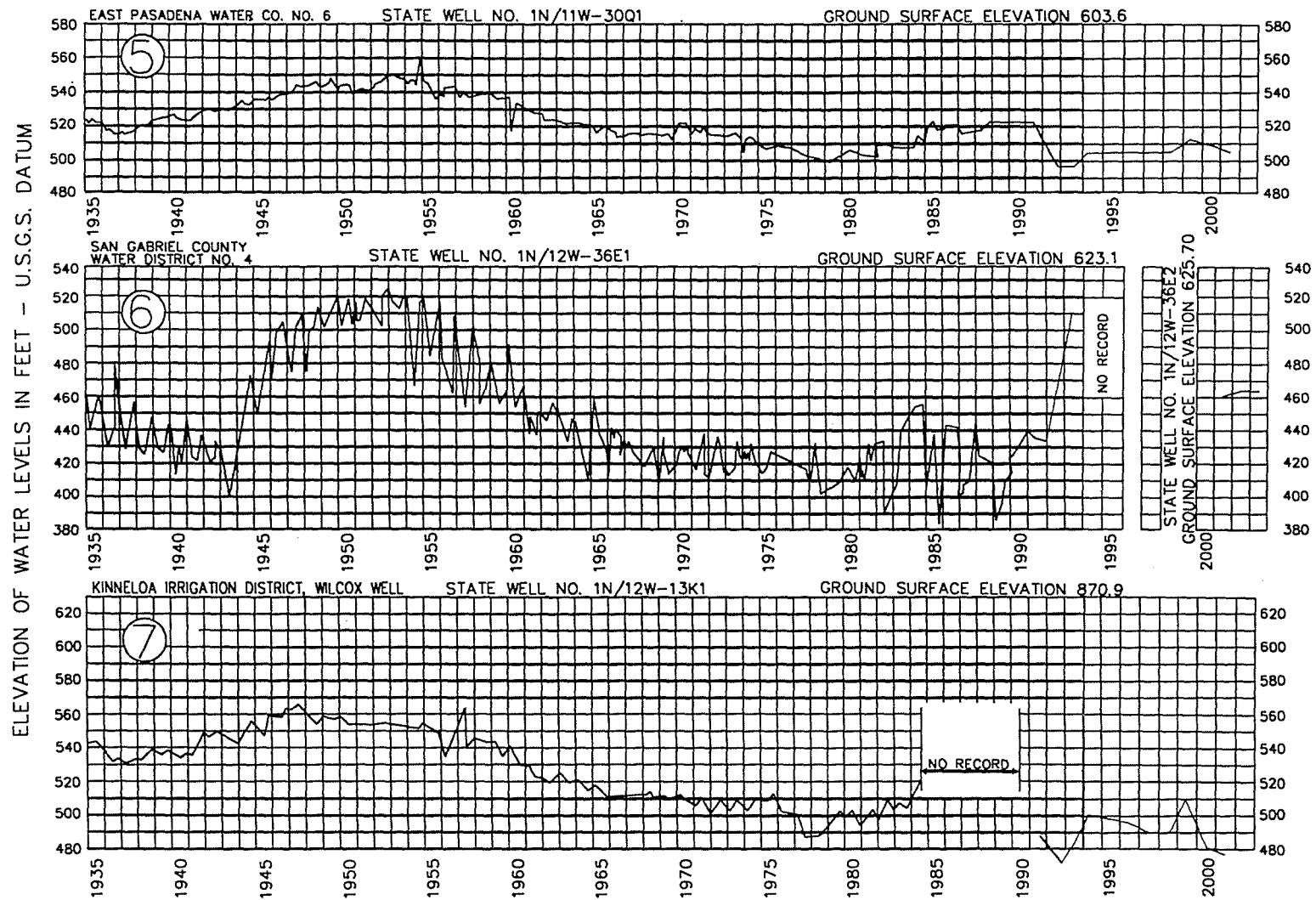
FIGURE 10b - FLUCTUATION OF WATER LEVELS AT WELLS IN THE PASADENA SUBAREA
