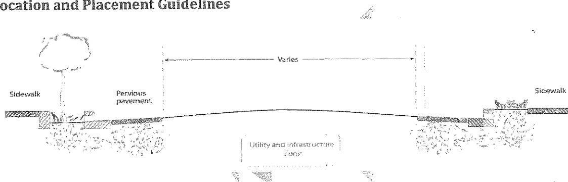
Figure 5: Possible pervious pavement design layout ( Model for Living Streets Design Manual, 2011 ).
