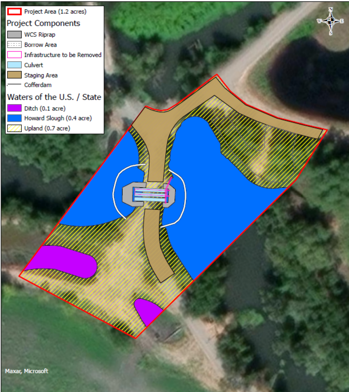
Figure 4. Project Components within Waters of the U.S. / State Howard Slough Water Control Structure Replacement Project
