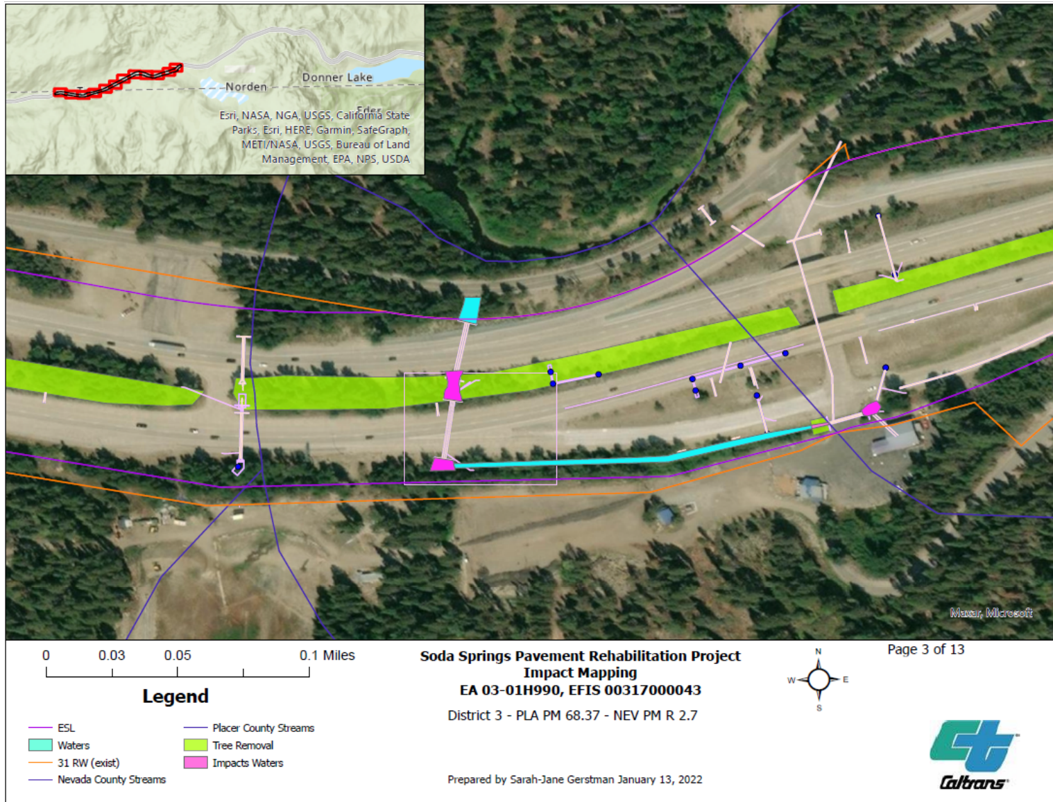
Figure 3: Project Impacts Map Drainage System #8
