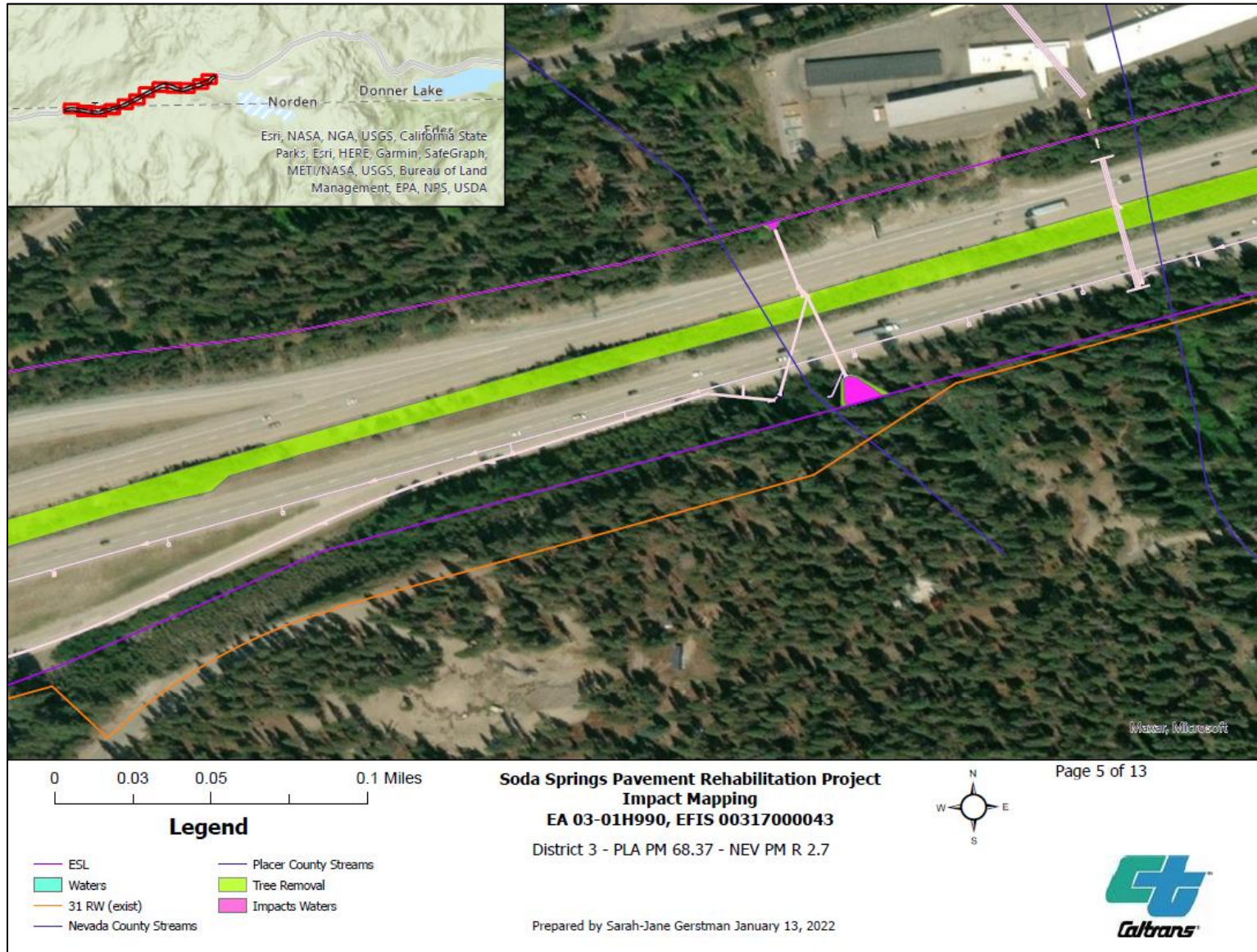
Figure 5: Project Impacts Map Drainage System #15
