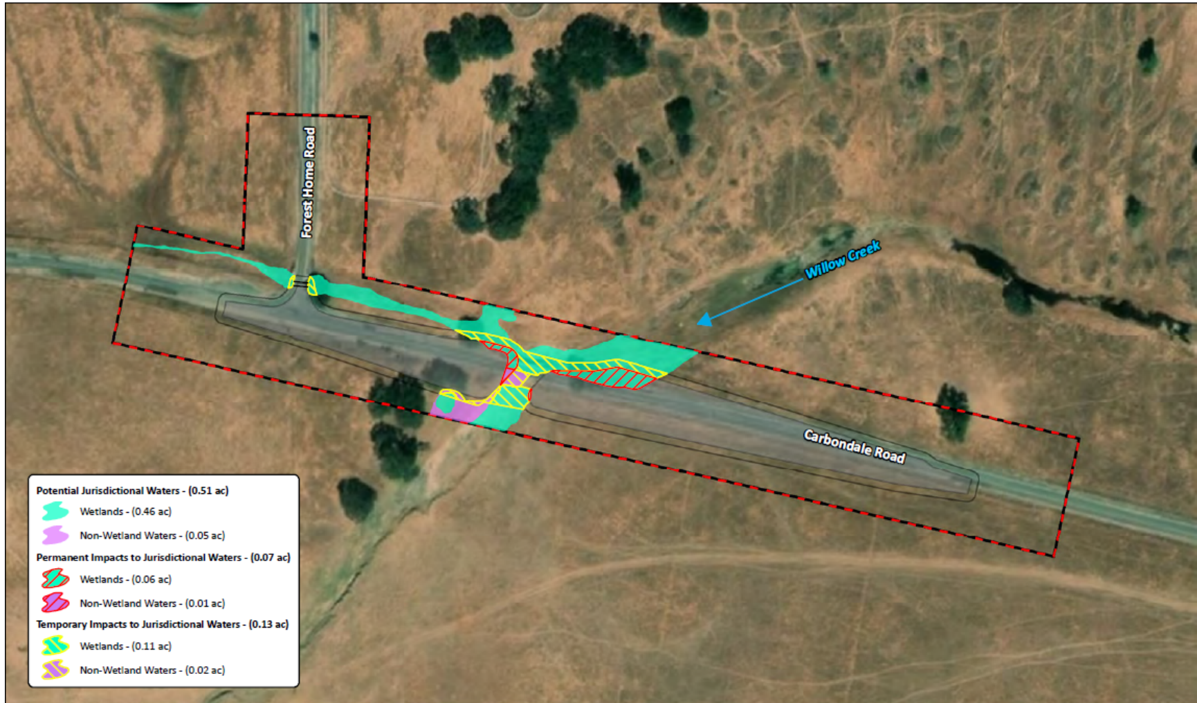
FIGURE 2 Impacts to Jurisdictional Waters Carbondale Road Bridge (26C0030) Replacement Project at Willow Creek
