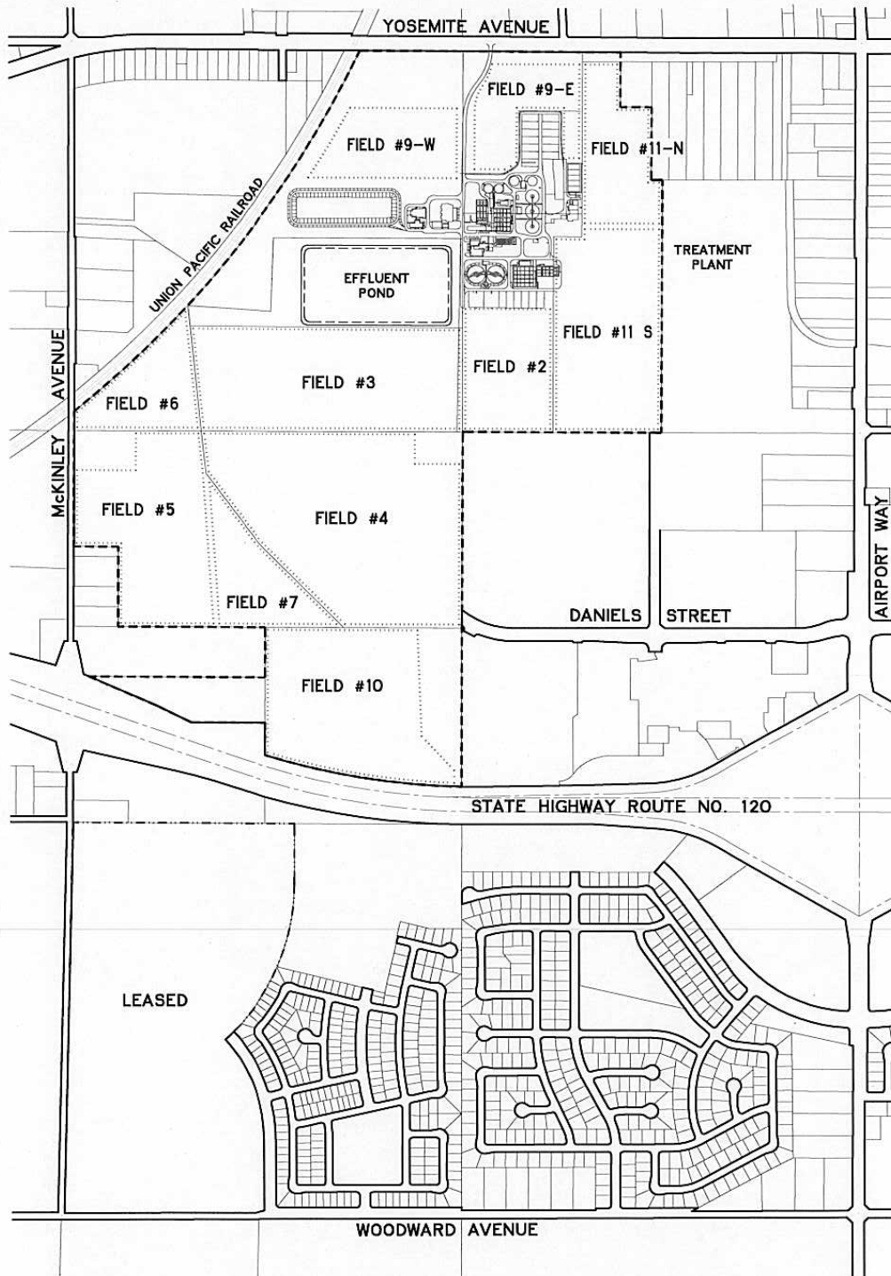
Figure 2 - Manteca WQCF Land Application Areas
