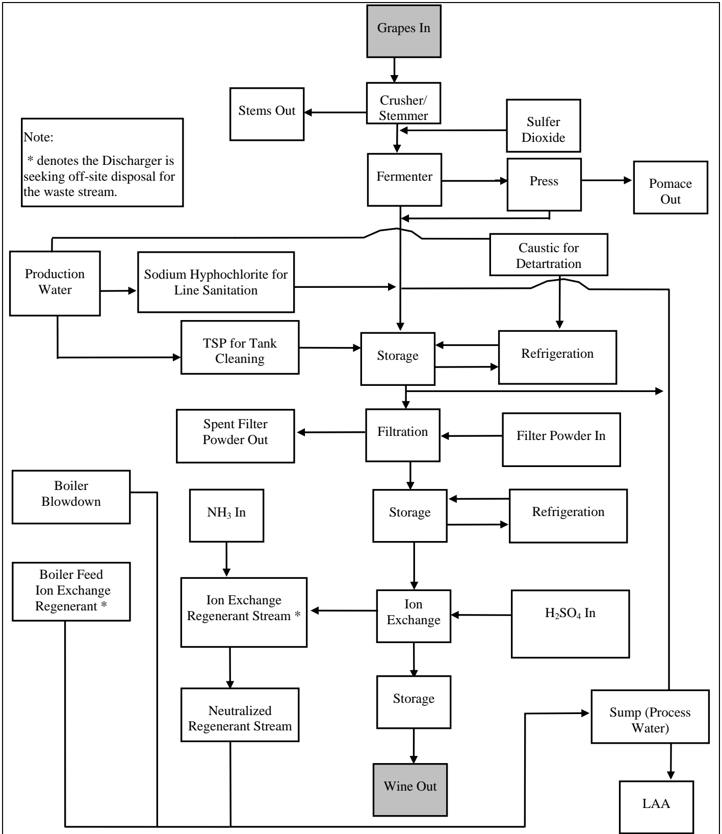
Drawing Reference: Figure 1, RWD 9/05 Kennedy Jenks Consultants WASTEWATER FLOW DIAGRAM BARREL TEN QUARTER CIRCLE, ESCALON CELLARS ESCALON, SAN JOAQUIN COUNTY
