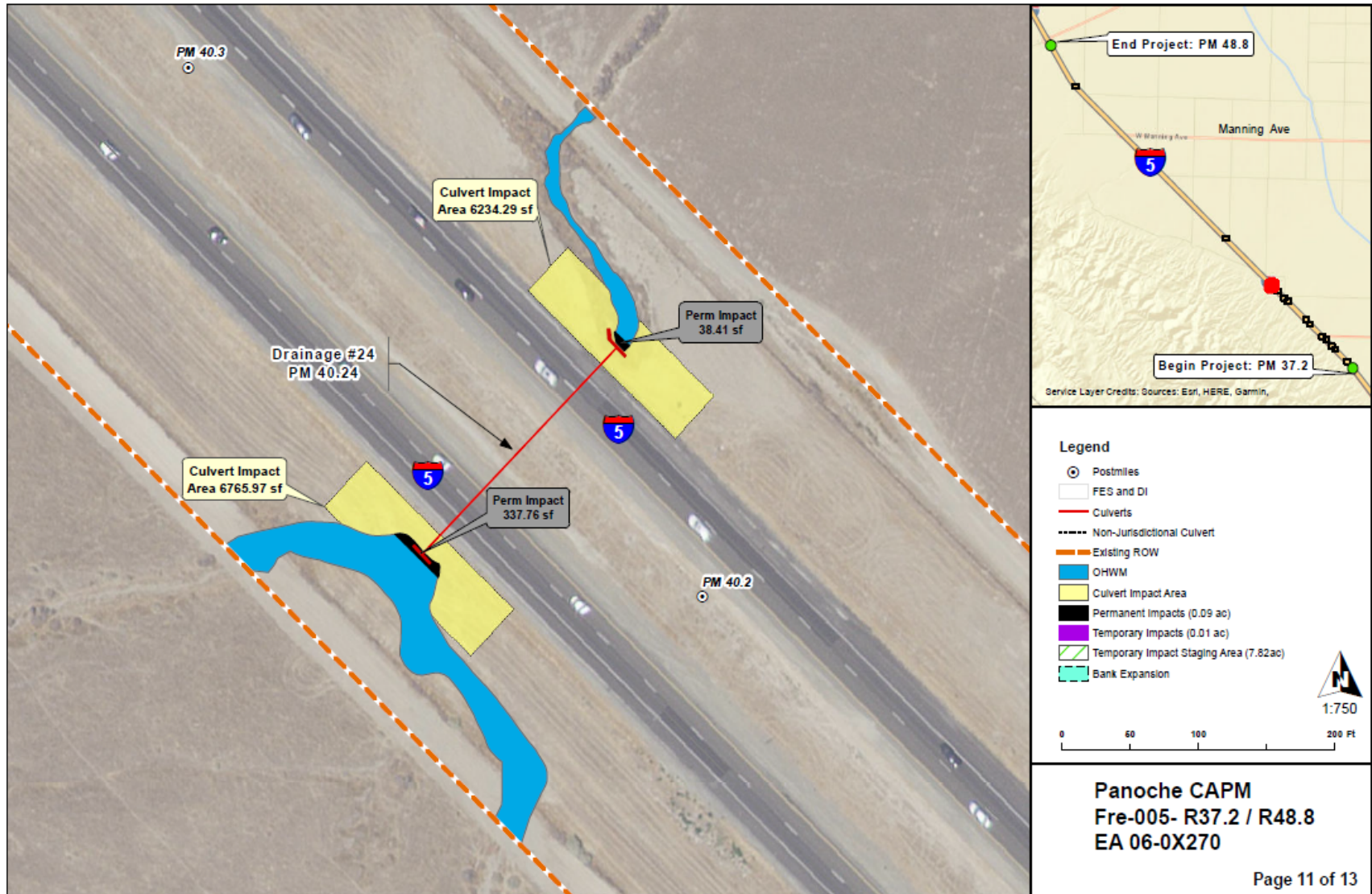
Figure 11. Project Location and Impacts Post Mile 40.24
