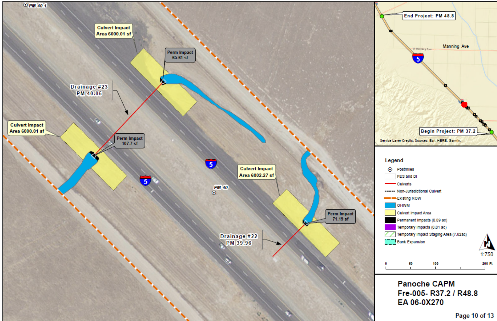
Figure 10. Project Location and Impacts Post Mile 40.05
