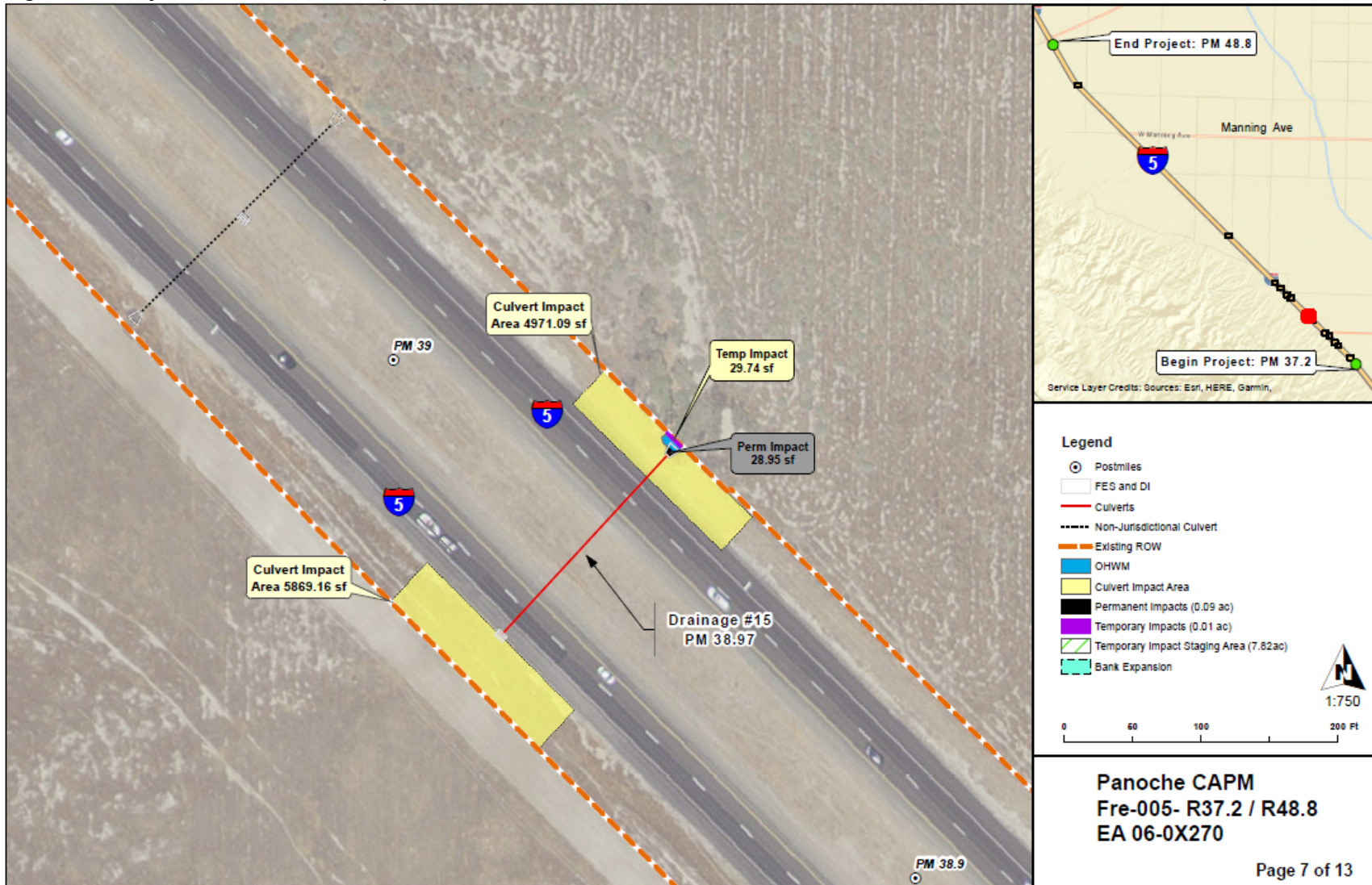
Figure 7. Project Location and Impacts Post Mile 38.97
