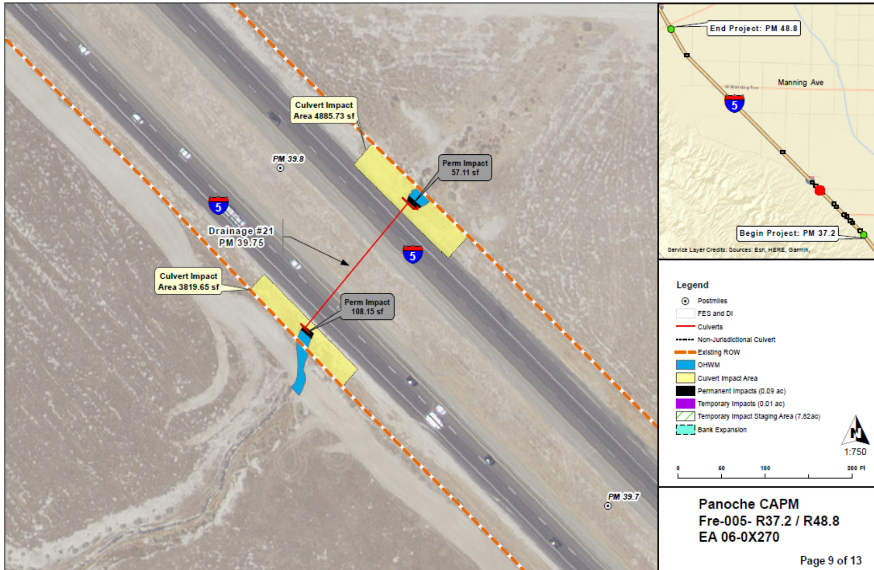
Figure 9. Project Location and Impacts Post Mile 39.75
