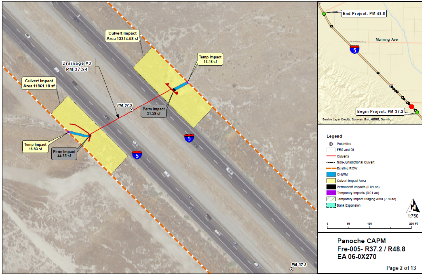
Figure 2. Project Location and Impacts Postmile 37.90
