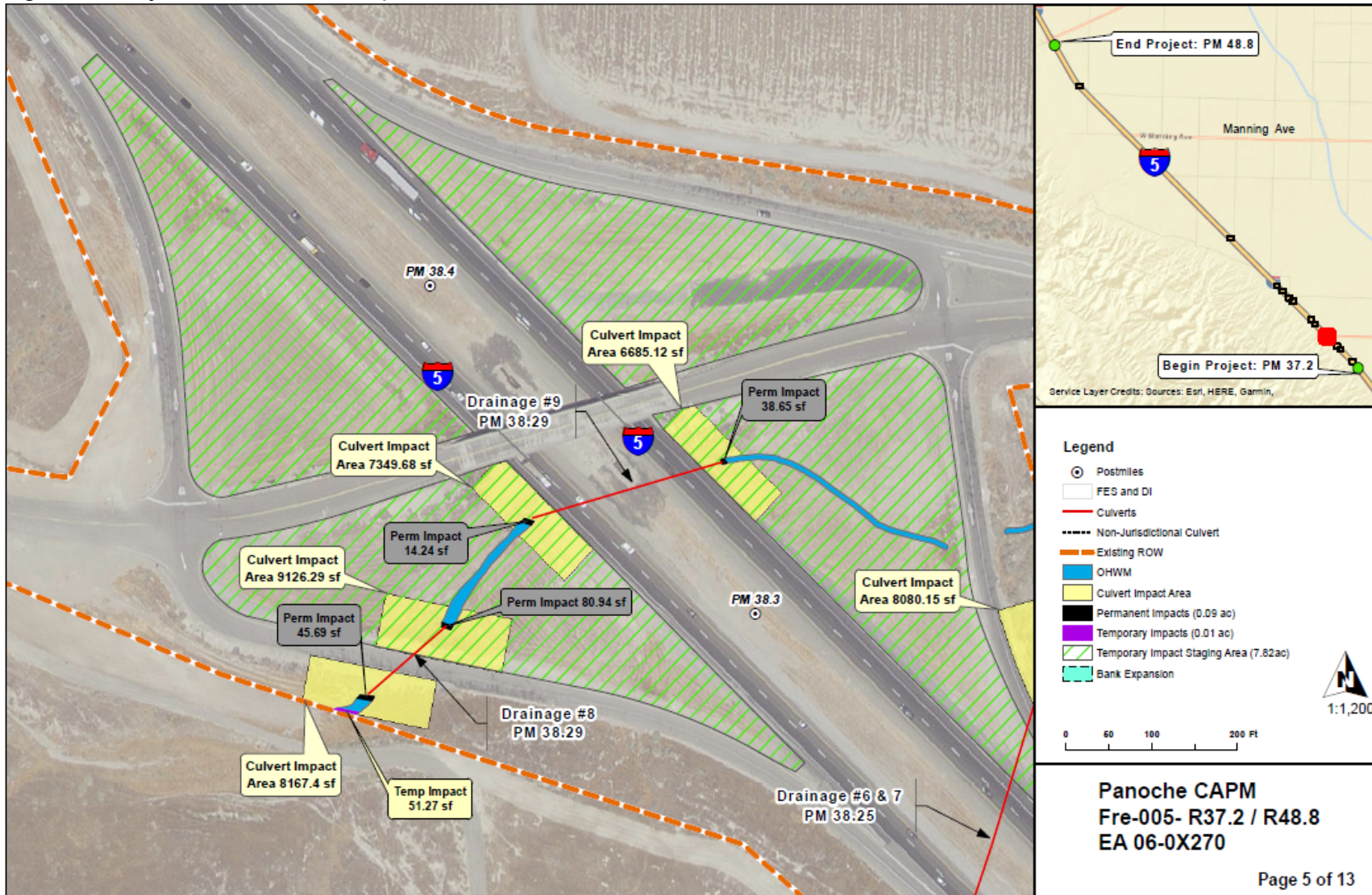
Figure 5. Project Location and Impacts Post Mile 38.29
