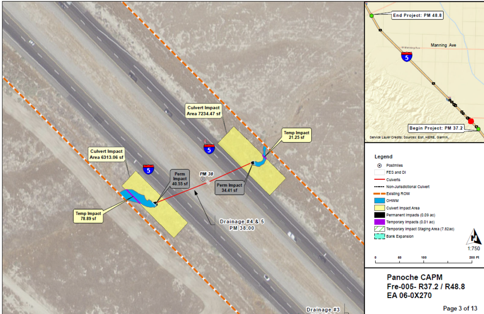
Figure 3. Project Location and Impacts Post Mile 38.00
