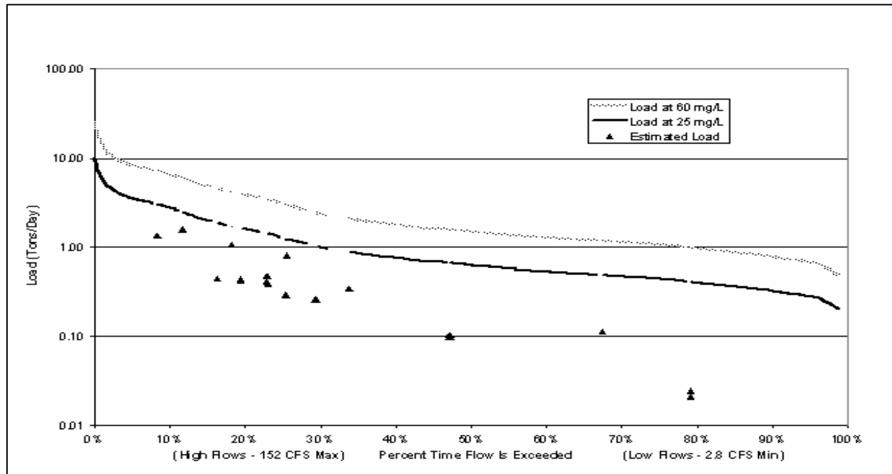
Figure 3-3. Load Duration Curve for Bronco Creek. Allowable loads at 25 and 60 mg/L SSC are shown as curved lines, and measured loads are triangles. Note that none of the measured loads exceed the allowable loads.
