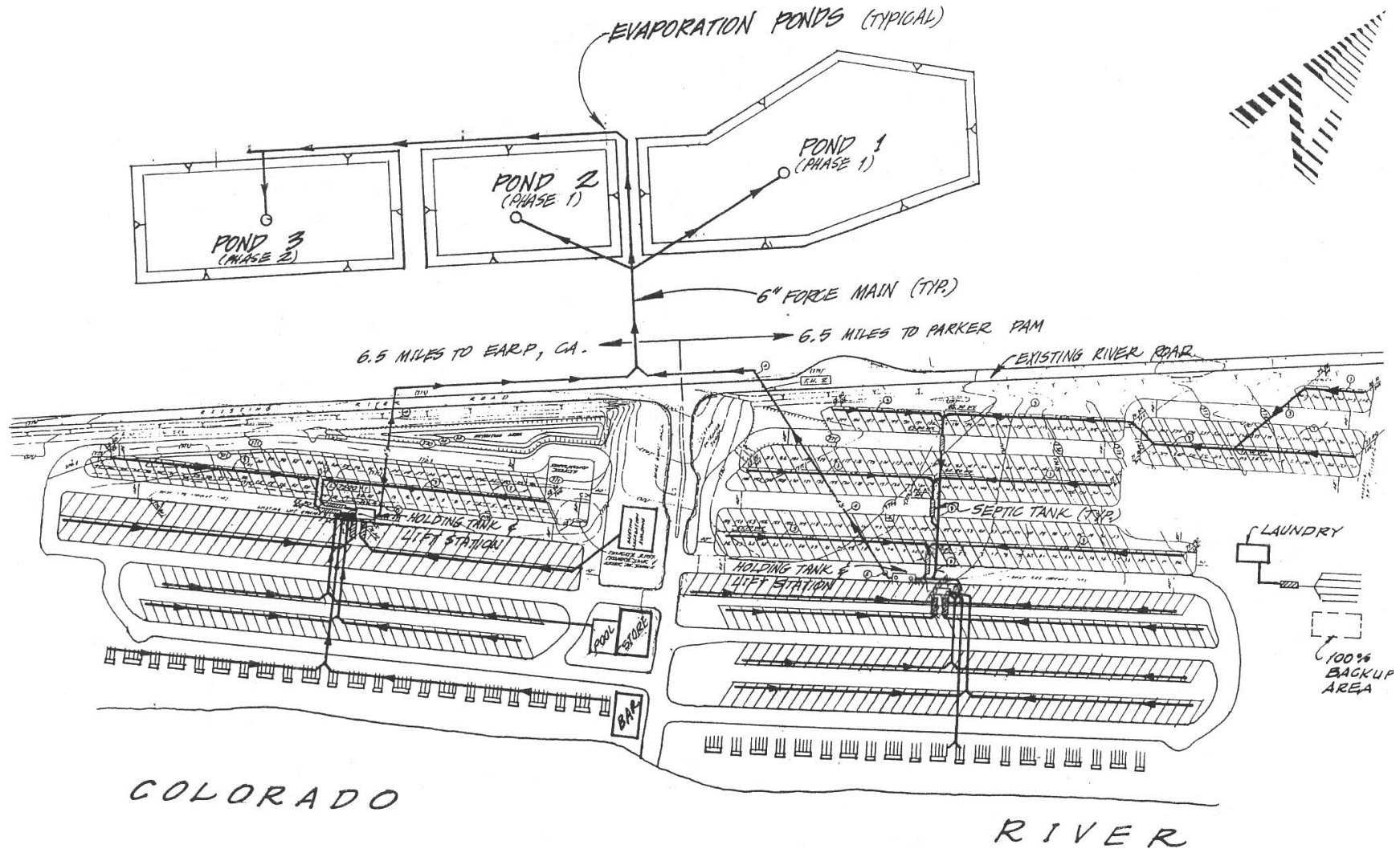
SITE MAP EMERALD COVE RESORT, L.L.C., OWNER/OPERATOR EMERALD COVE RESORT SEPTIC TANK/EVAPORATION BASIN DISPOSAL FACILITIES Northeast of Earp - San Bernardino County
