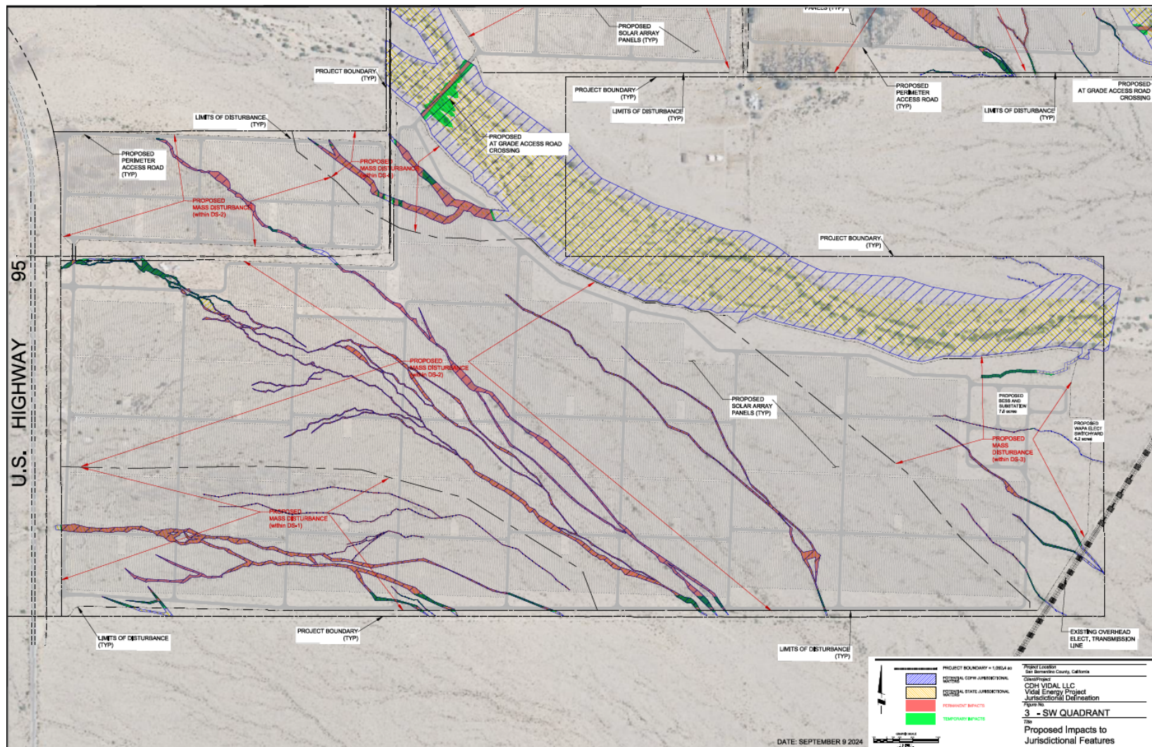
Figure 4: Vidal Energy Project site plan and impacts to jurisdictional features (SW quadrant)
