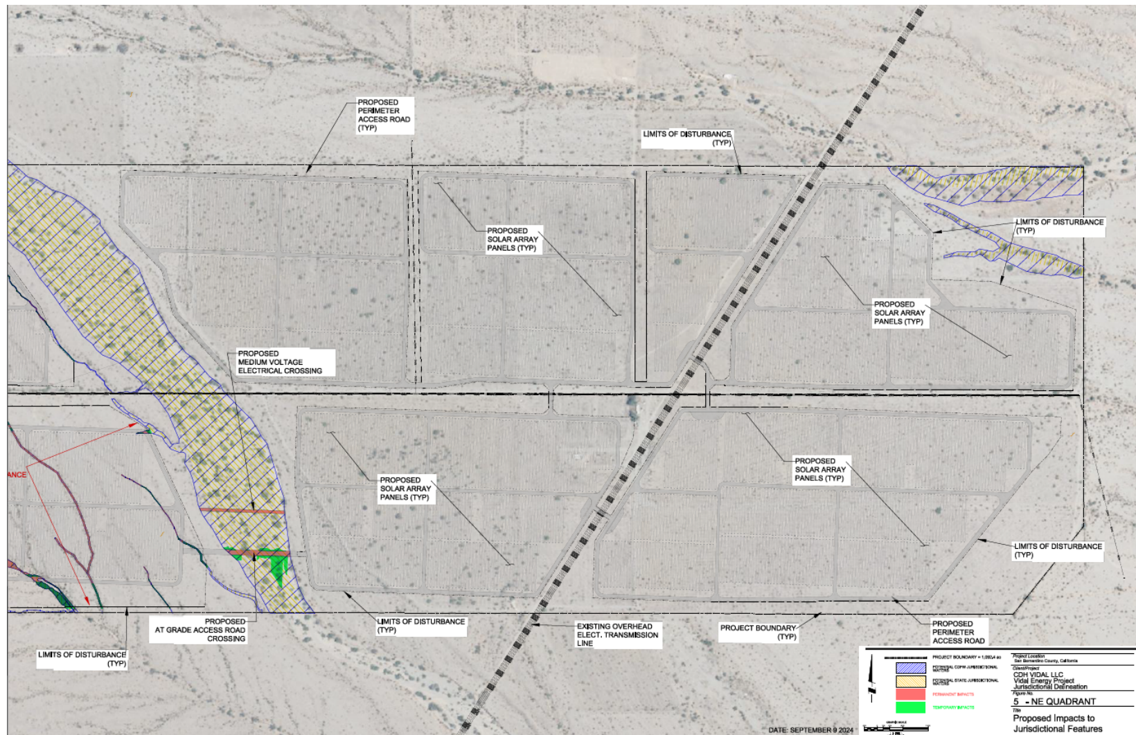
Figure 6: Vidal Energy Project site plan and impacts to jurisdictional features (NE quadrant)
