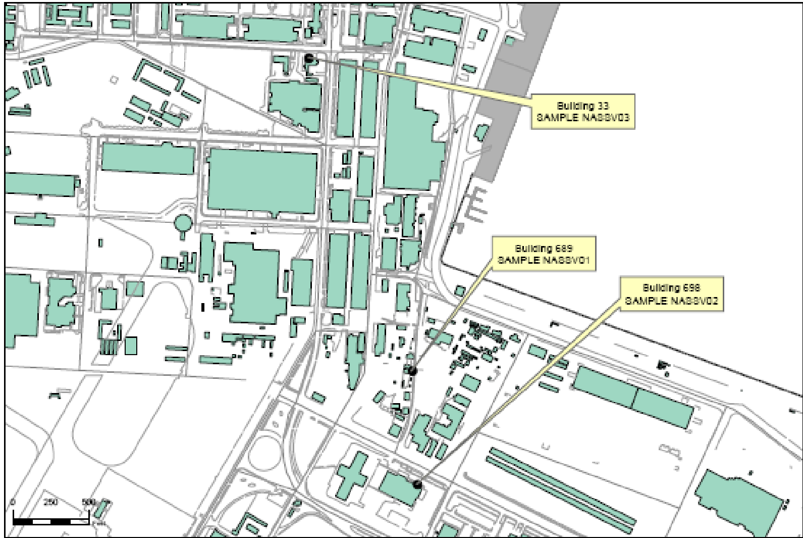
Figure B-9. Steam Vault Locations at NASNI
