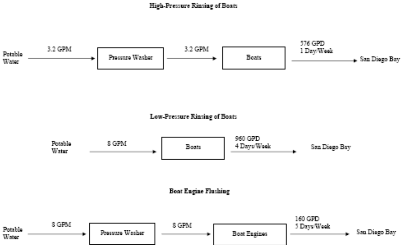
Figure C-10. Boat Rinsing Line Drawing
