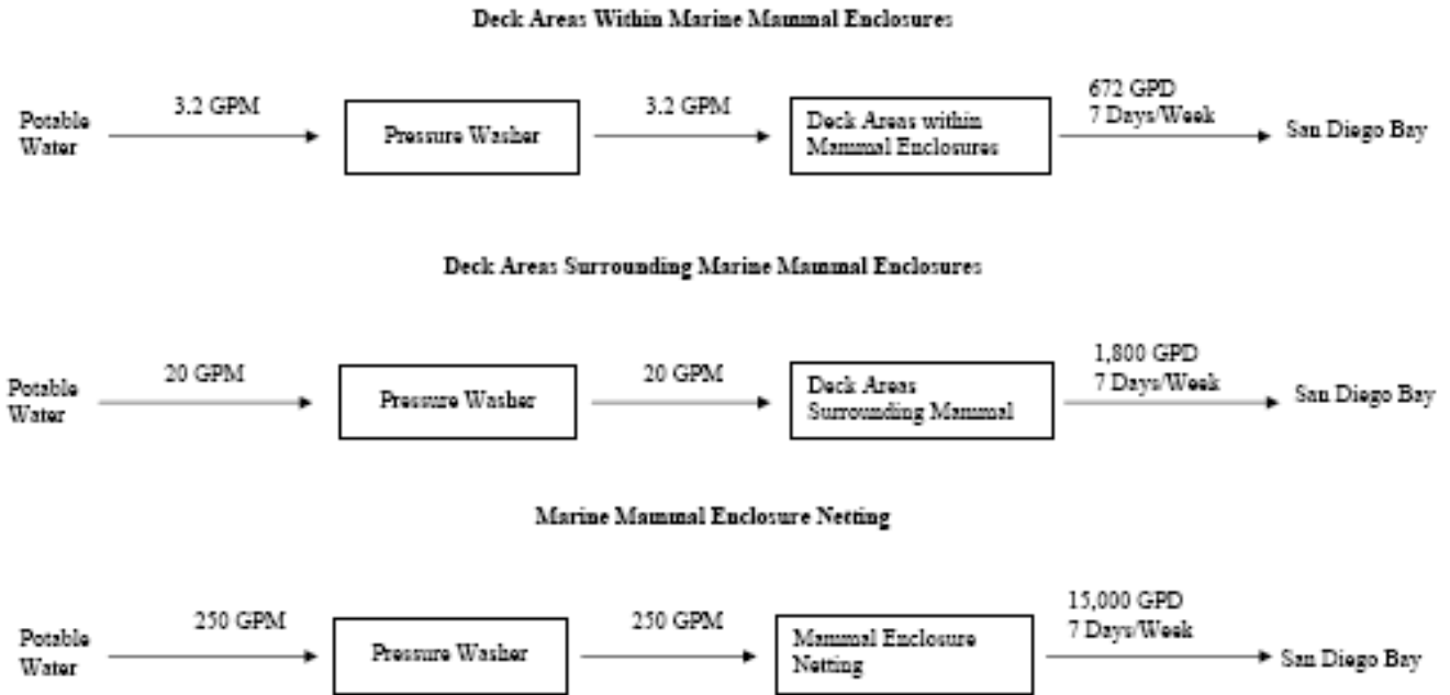
Figure C-12. Marine Mammal Enclosure Cleaning Line Drawing
