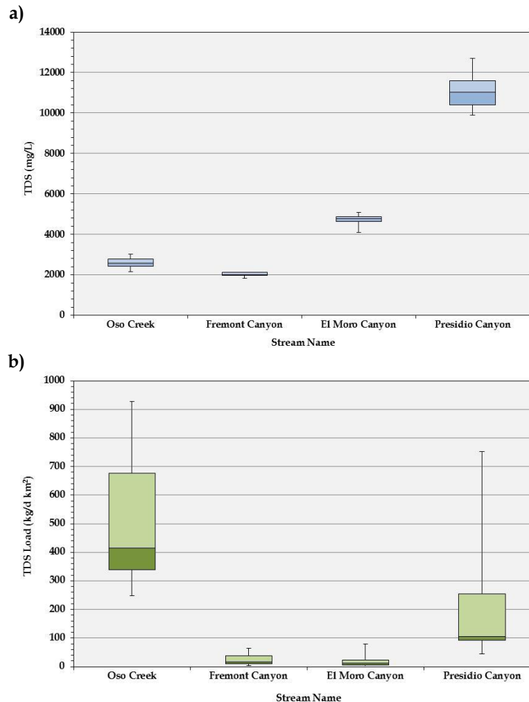
Figure 2.4.3: Ranges of dissolved solid concentrations (a) and loads (b) in Oso Creek in comparison to three reference streams of similar geology.
