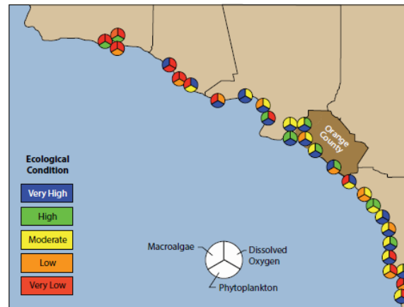
Figure 2.5.2: Almost all estuarine segments in the Southern California Bight show some degradation on at least one of the three response indicators of eutrophication: macroalgal cover, phytoplankton, and dissolved oxygen concentration. Adapted from Bight '08 program data.
